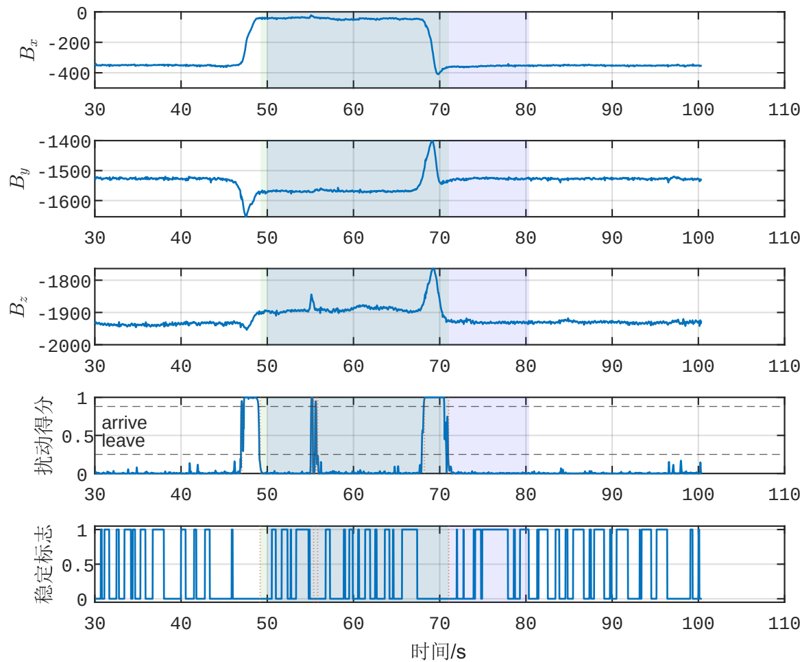
B类波形示例 (GT#1, N_{ev}=3 , stable=0.39, pr=0.110)
