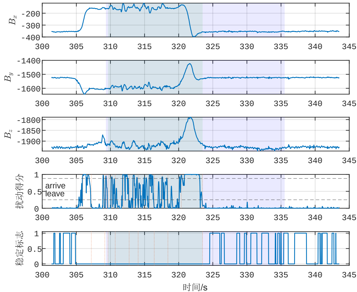
B类波形示例 (GT#4, N_{ev}=7 , stable=0.20, pr=0.278)
