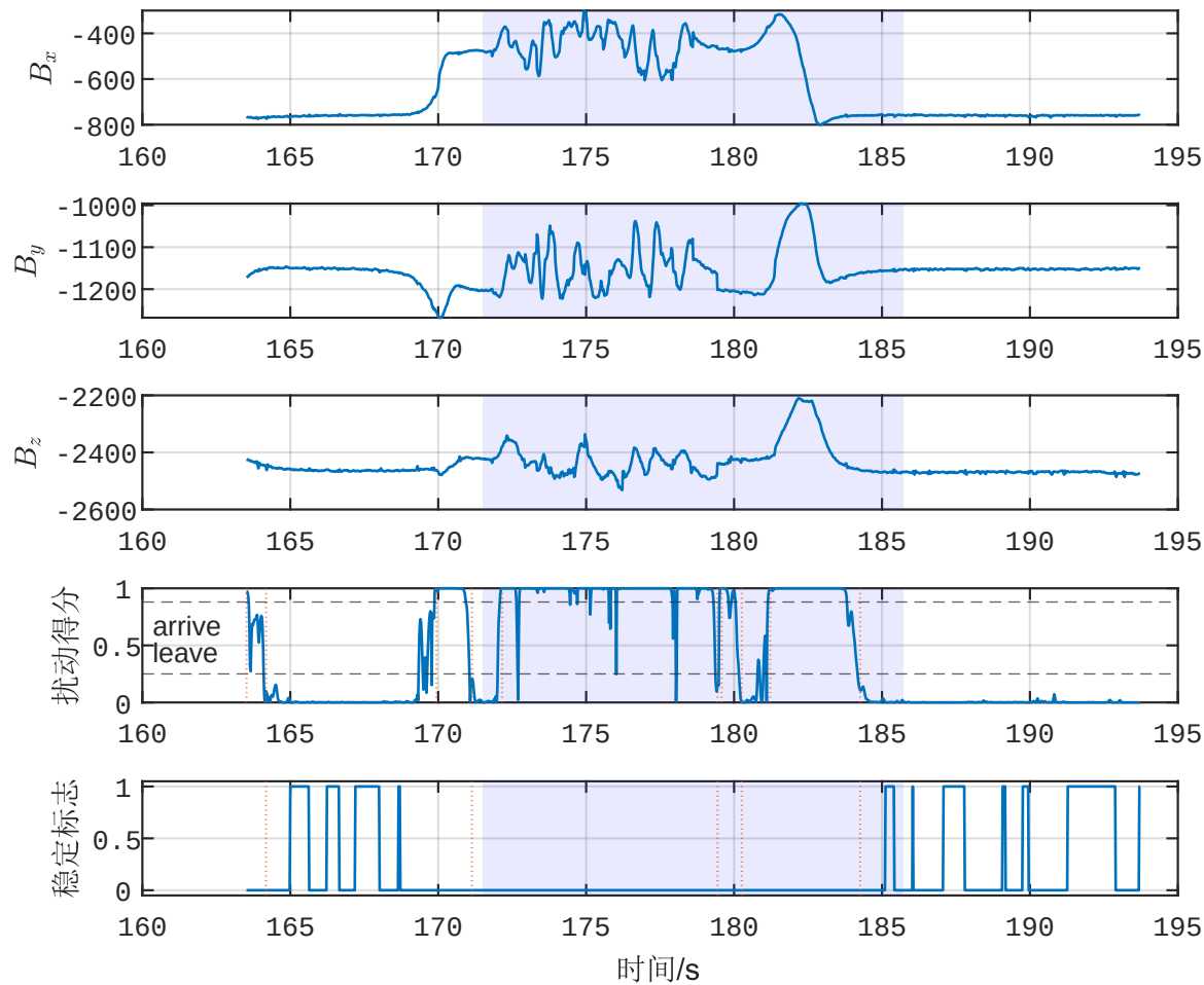
B类波形示例 (GT#3, N_{ev}=3 , stable=0.02, pr=0.760)
