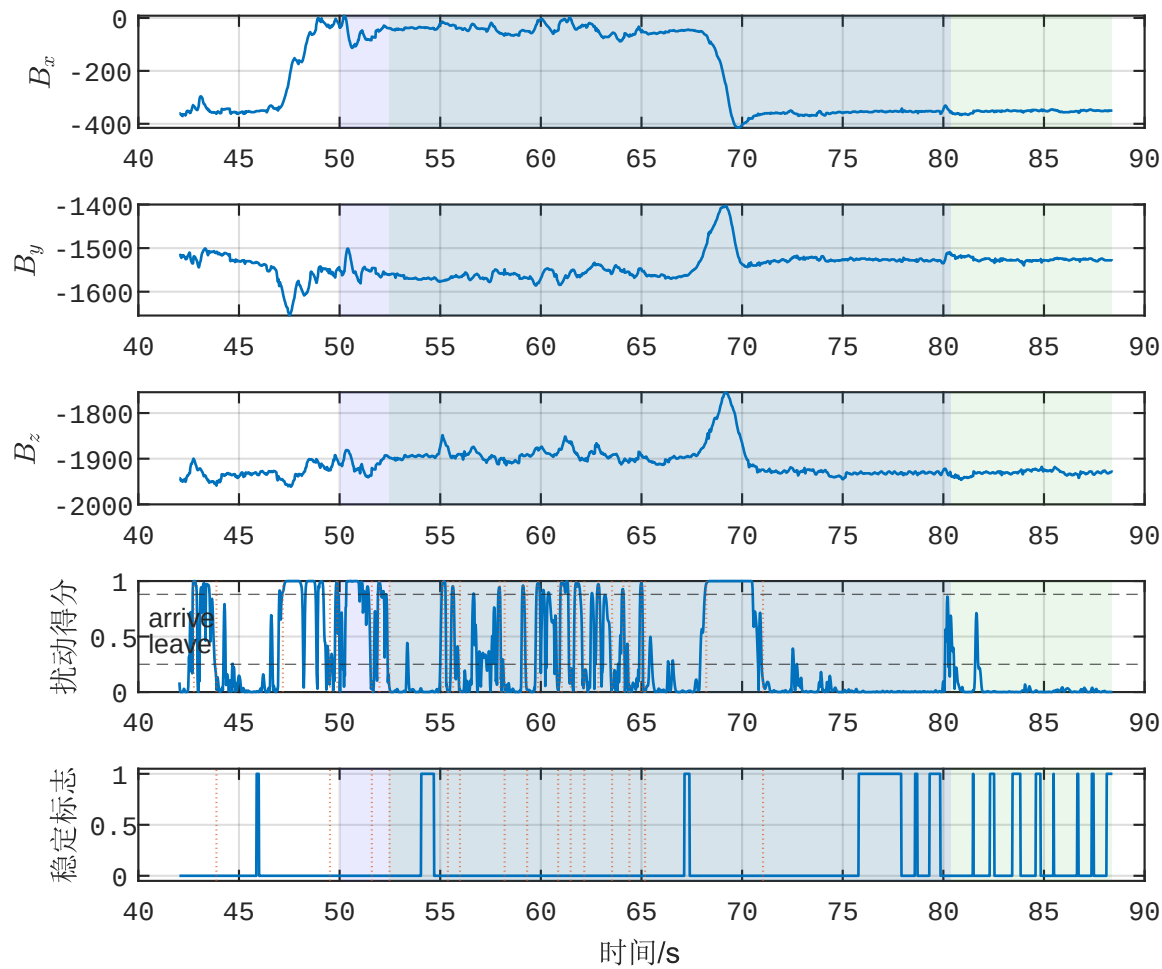
C类波形示例 (GT#1, N_{ev}=13 , stable=0.12, pr=0.298)
