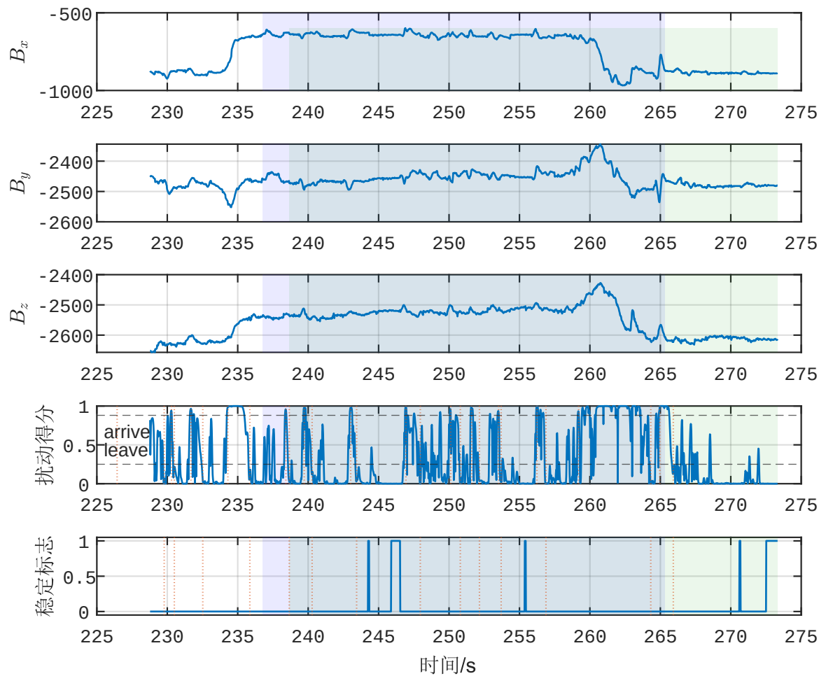
C类波形示例 (GT#4, N_{ev}=10 , stable=0.03, pr=0.370)
