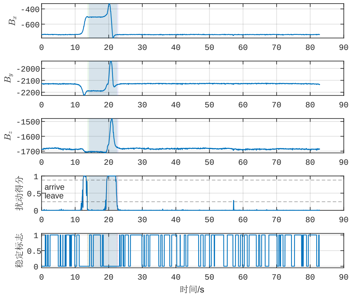
D类波形示例 (GT#1, N_{ev}=1 , stable=0.34, pr=0.356), drift=30.26
