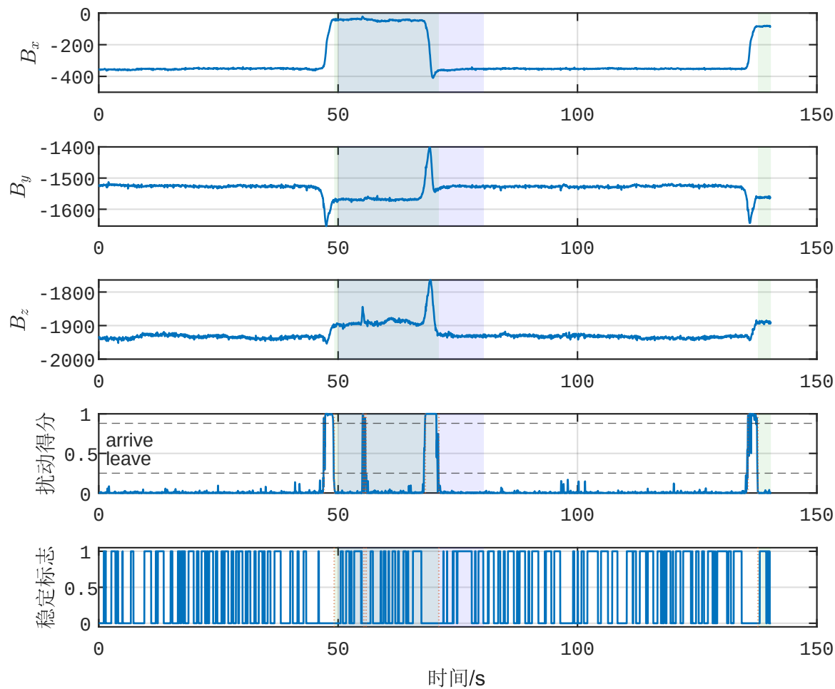
D类波形示例 (GT#1, N_{ev}=3 , stable=0.39, pr=0.110), drift=26.28
