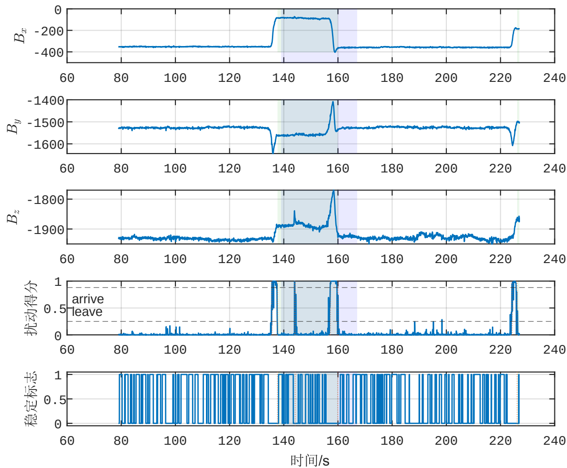
D类波形示例 (GT#2, N_{ev}=2 , stable=0.34, pr=0.124), drift=31.78
