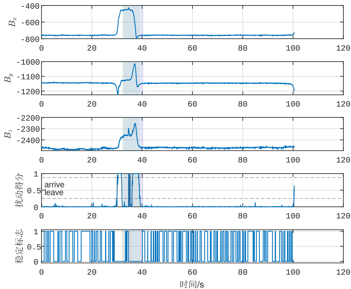
D类波形示例 (GT#1, N_{ev}=3 , stable=0.15, pr=0.428), drift=20.69
