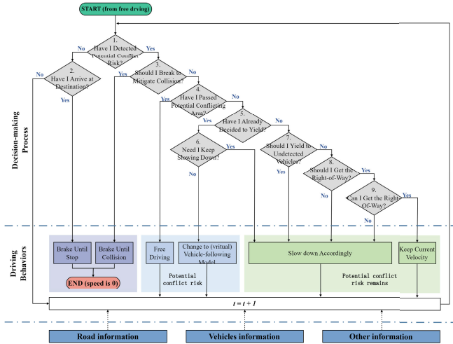
Fig. 8. Flowchart of the communication-decision model for RoW in proactive collision prevention for AVs. The model outlines a rule-based, nine-step paradigm that facilitates clear and efficient communication between AVs and human drivers, ensuring safe and coordinated interactions on the road.
