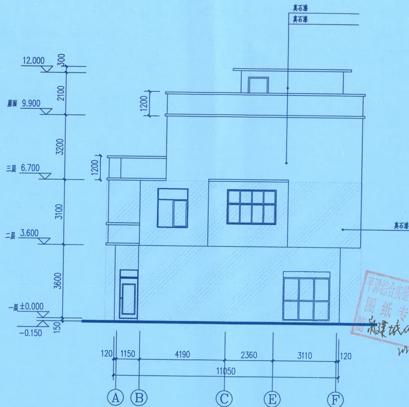
(A)~(F)轴立面图 1:100 (拟建)
