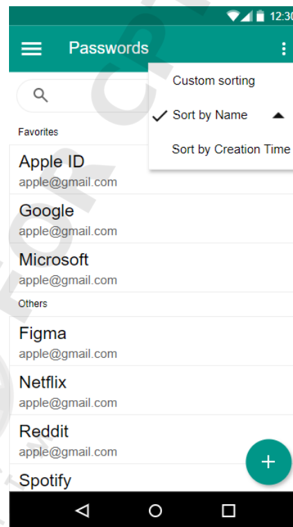
Passwords Page
