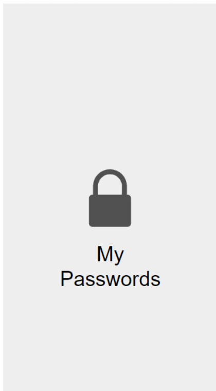
Launch Page
