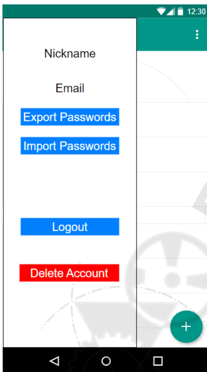
Drawer
