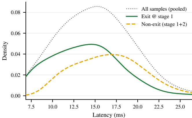
Naive Latency by Exit Class ( \lambda=1490 req/s)
