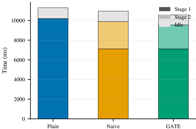
GPU Time Breakdown
