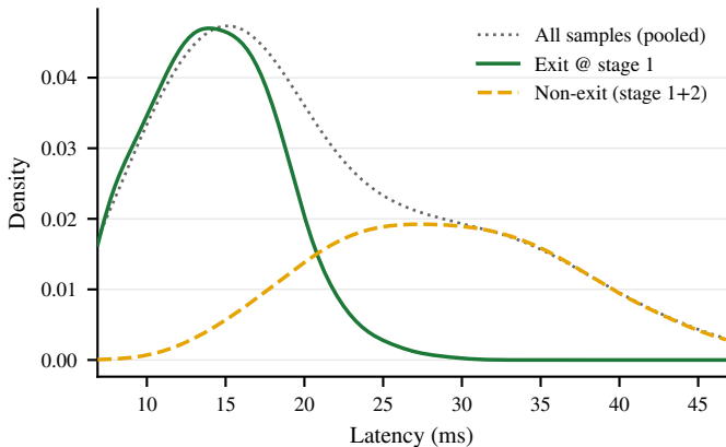
GATE ( bs_2 = 16 ) Latency by Exit Class ( \lambda = 1540 req/s)
