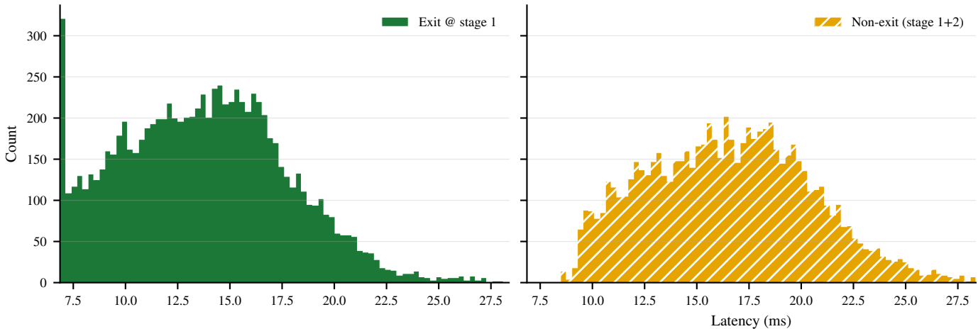
Naive Latency by Exit Class ( \lambda=1485 req/s)
