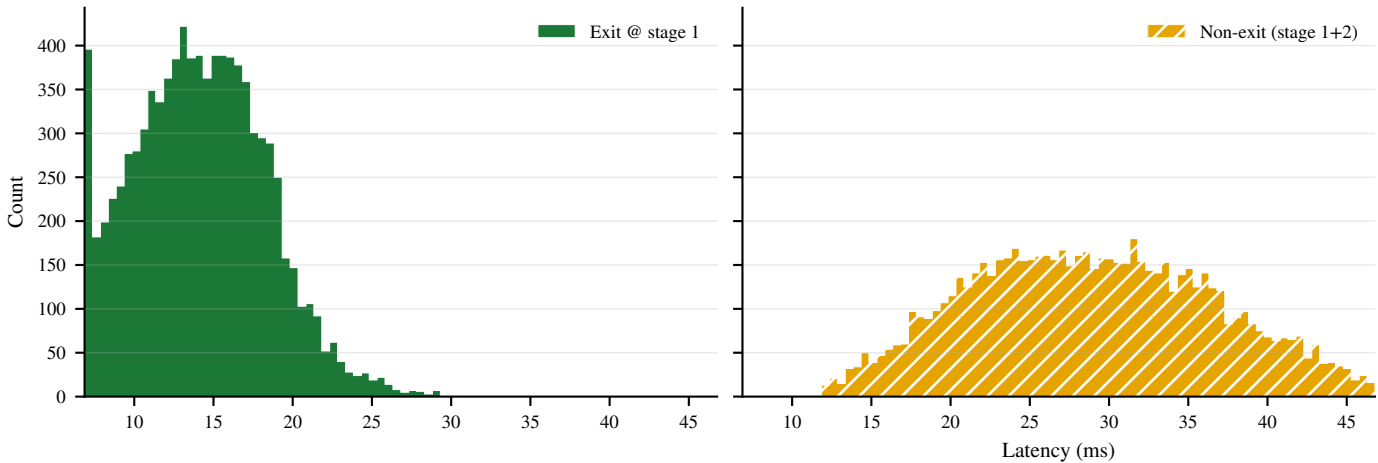
GATE ( bs_2 = 16 ) Latency by Exit Class ( \lambda = 1540 req/s)
