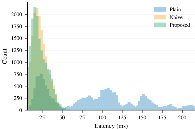
Latency Distribution at a Shared Load ( \lambda=1630 req/s)
