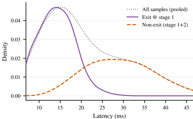
Proposed ( bs_2 = 16 ) Latency by Exit Class ( \lambda = 1555 req/s)
