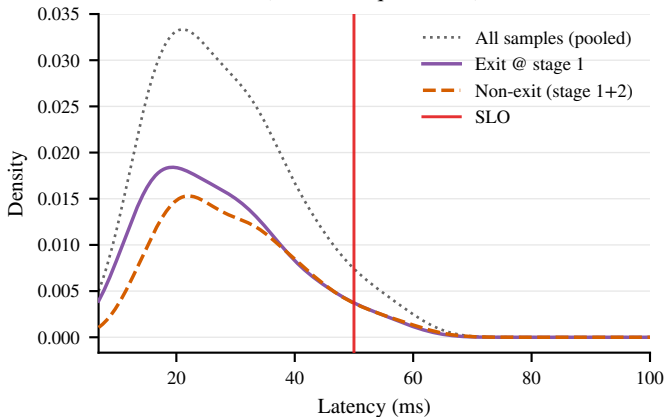
Naive Latency by Exit Class ( \lambda=1650 req/s, shared)
