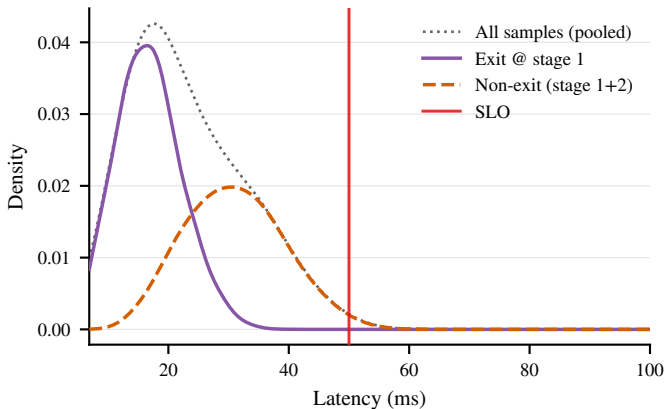
Proposed ( bs_2 = 16 ) Latency by Exit Class ( \lambda = 1650 req/s, shared)
