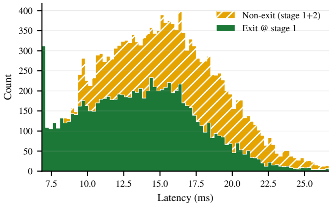
Naive Latency by Exit Class ( \lambda=1500 req/s)
