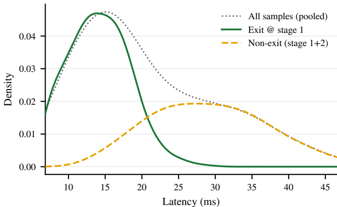
GATE ( bs_2 = 16 ) Latency by Exit Class ( \lambda = 1550 req/s)
