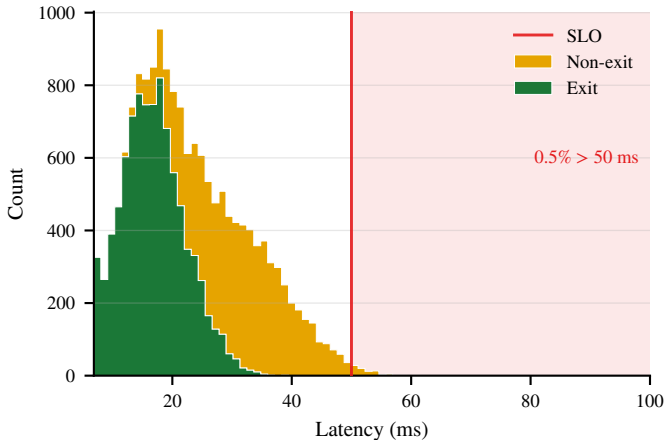
GATE ( bs_2 = 16 )
