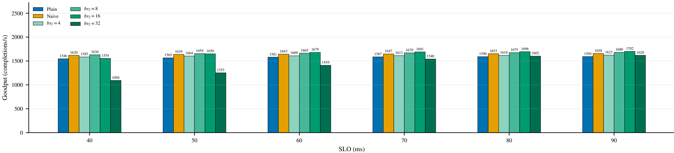
Peak Goodput
