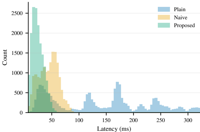
Latency Distribution at a Shared Load ( \lambda=1650 req/s)
