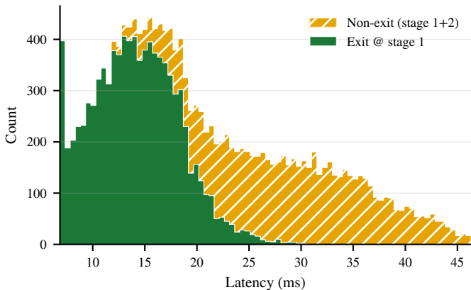
GATE ( bs_2 = 16 ) Latency by Exit Class ( \lambda = 1560 req/s)
