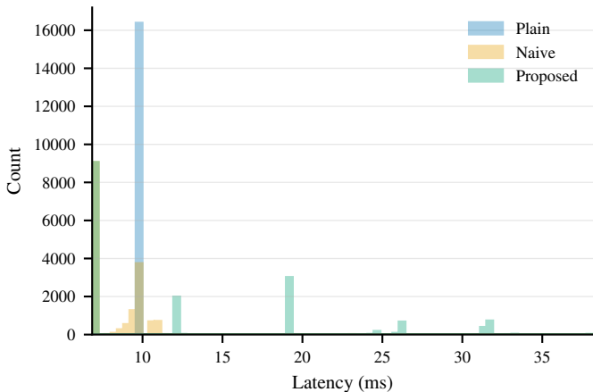
Latency Distribution at a Shared Load (saturated)
