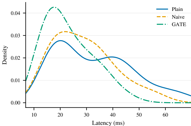
Latency Distribution at Per-Runtime Loads
