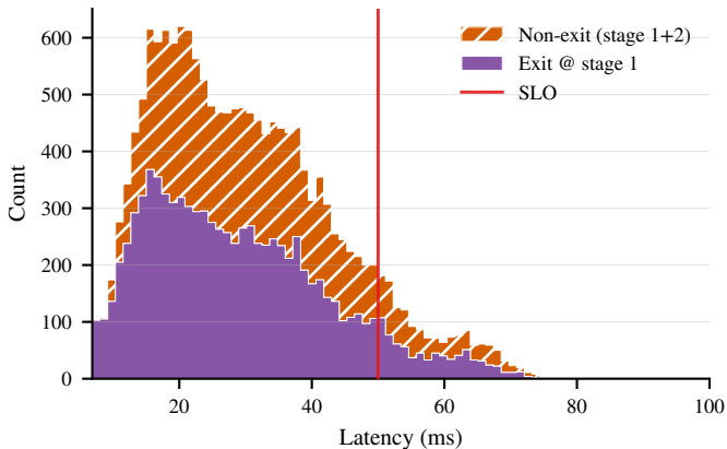
Naive Latency by Exit Class ( \lambda=1650 req/s, shared)
