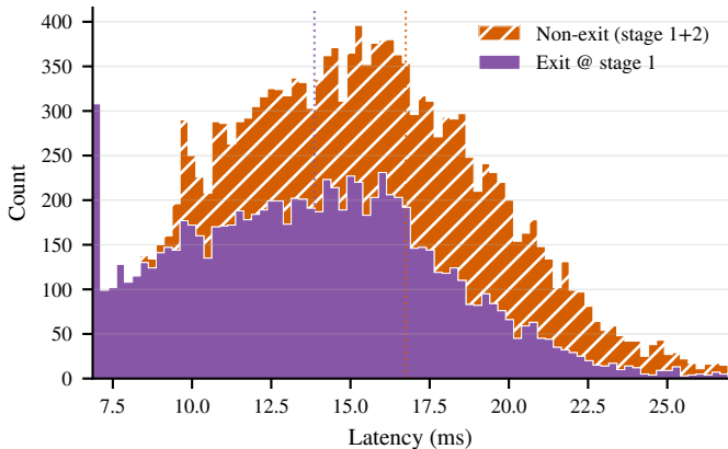
Naive Latency by Exit Class ( \lambda=1485 req/s)
