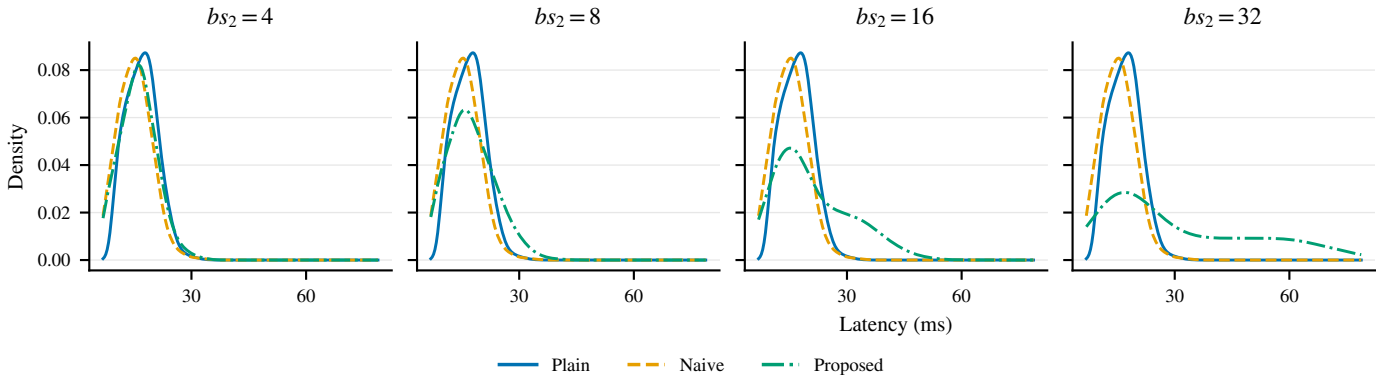
Latency Distribution
