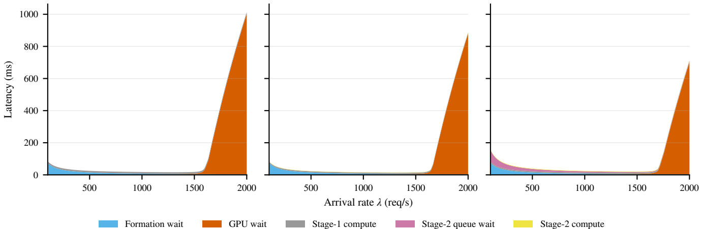
Proposed
