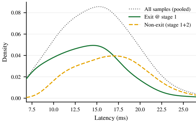
Naive Latency by Exit Class ( \lambda=1495 req/s)
