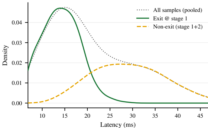
GATE ( bs_2 = 16 ) Latency by Exit Class ( \lambda = 1545 req/s)
