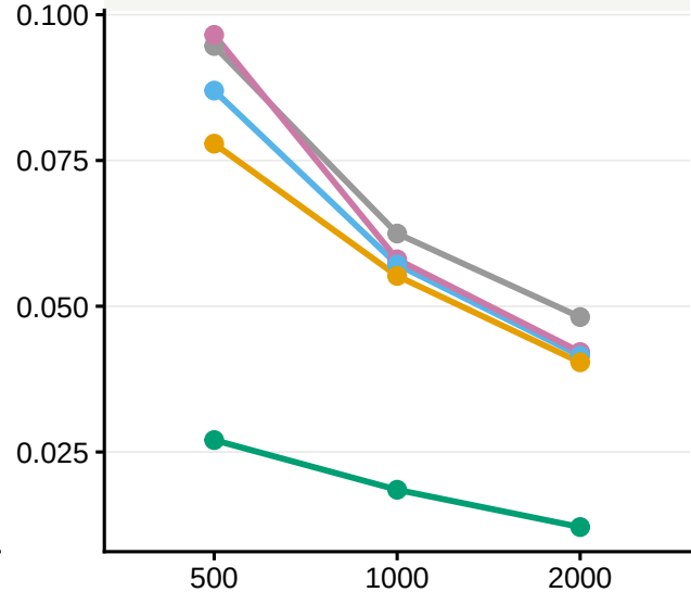
Polarized Mixture
