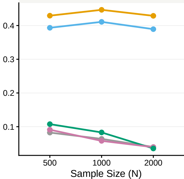
Heteroskedastic
