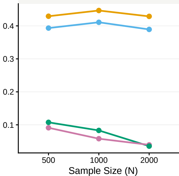
Heteroskedastic
