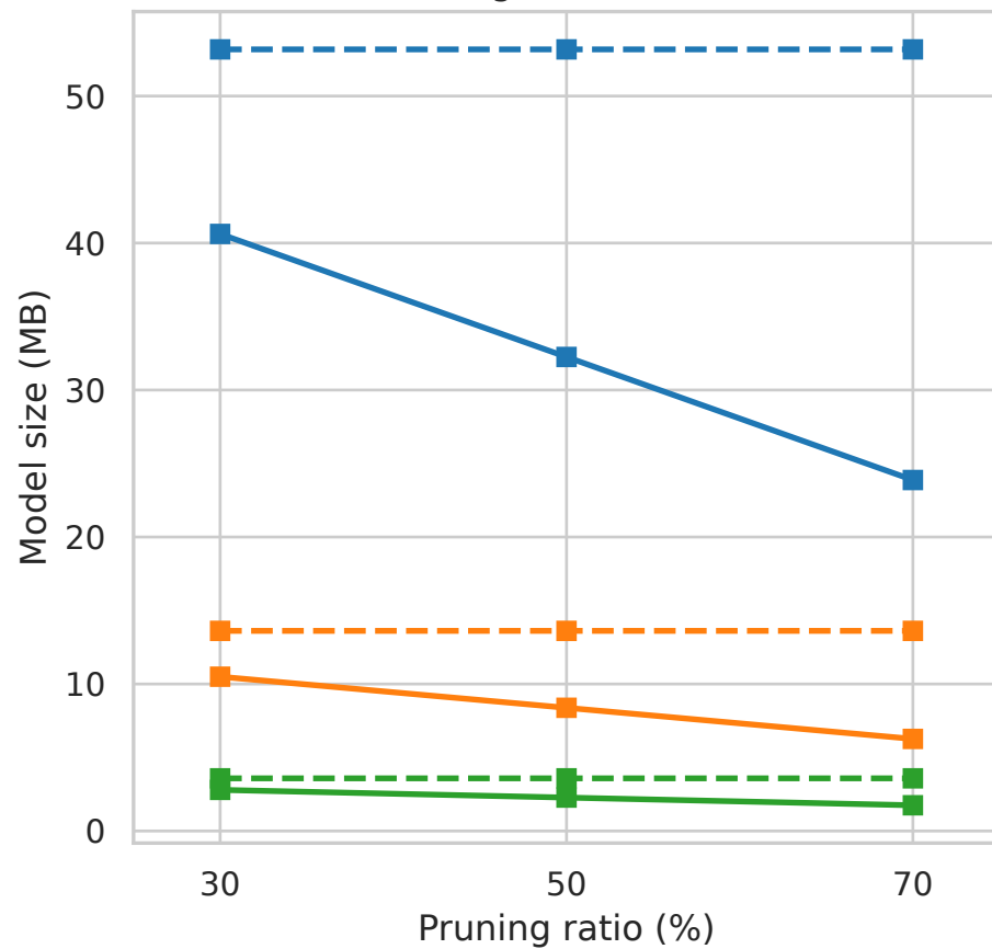
H3 Pruning: Model size (MB)
