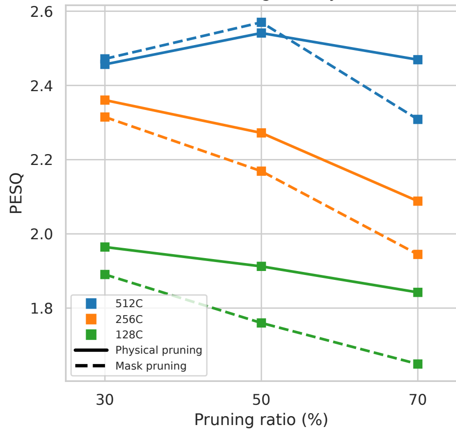
H3 Pruning: Quality
