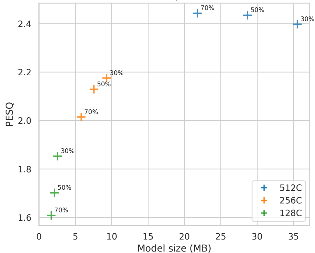
H4 Combined: Quality vs Model size (MB)
