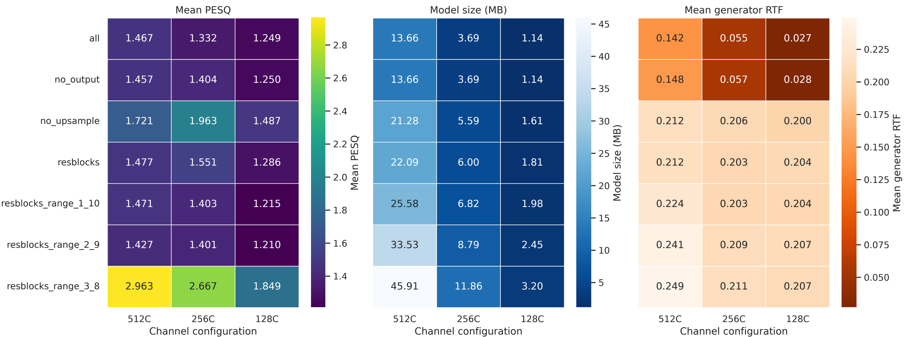
Quantization variant
