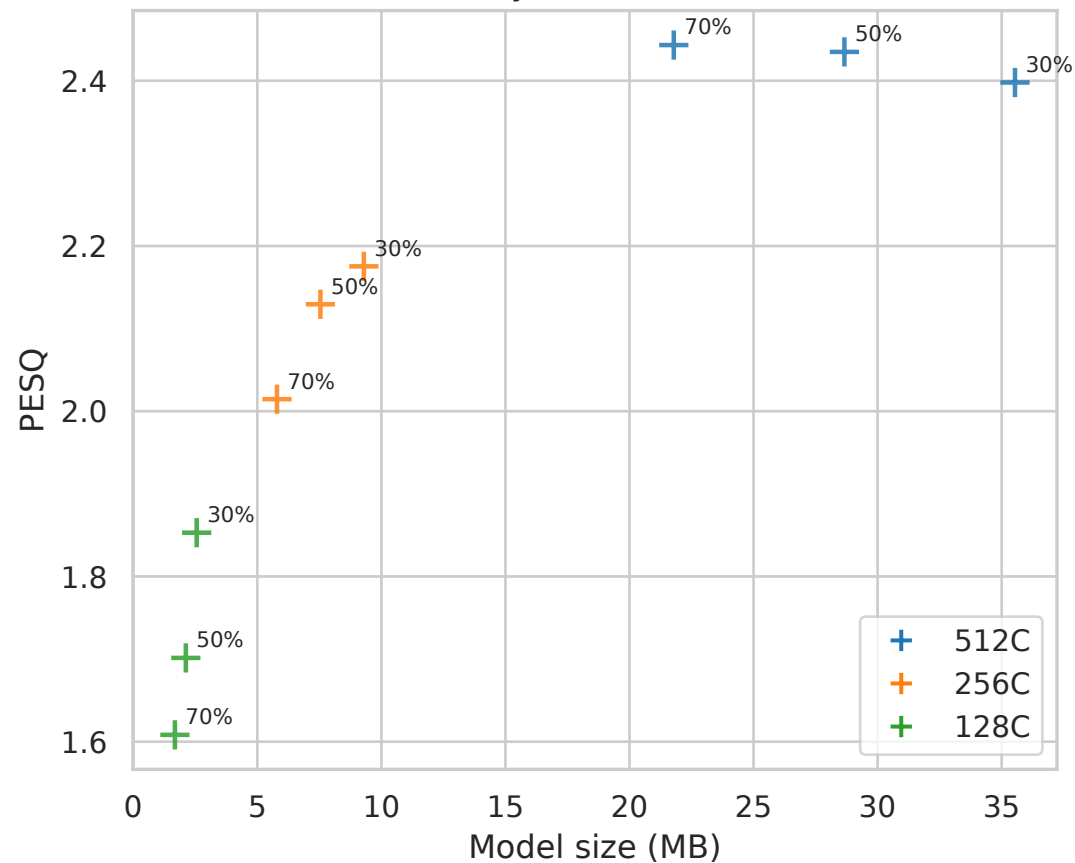
H4: Quality vs Model size (MB)
