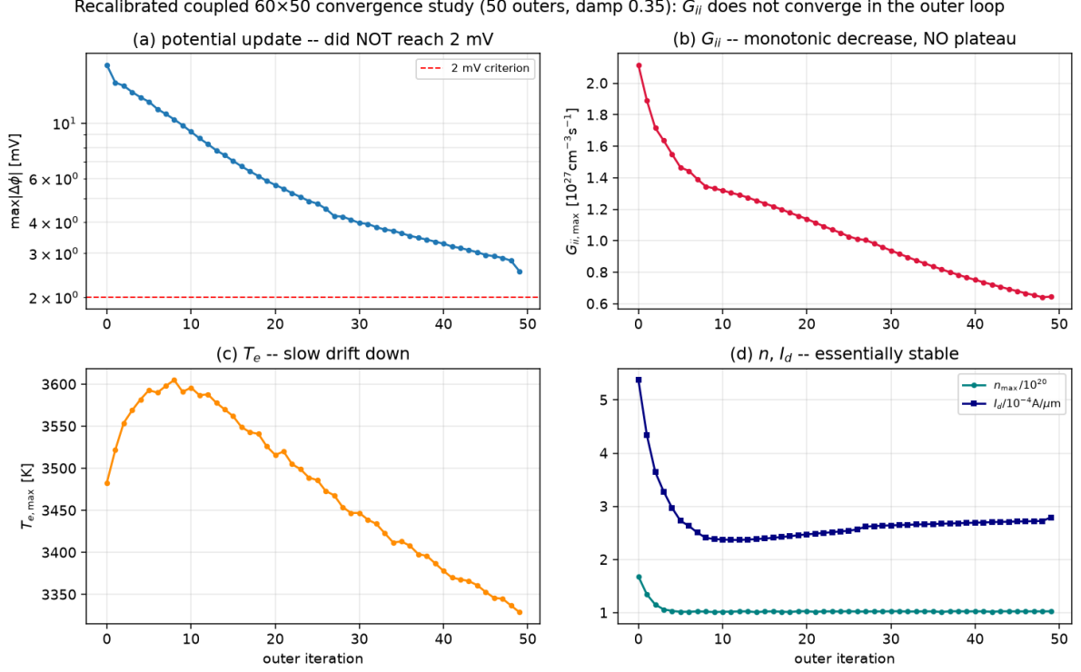
Figure 3: Recalibrated coupled 60×50 convergence study (50 outer iterations, \phi -damping 0.35). (a) \max|\Delta\phi| falls to 2.5 mV, short of the 2 mV criterion; (b) G_{ii,\max} decreases monotonically with no plateau — not converged in the outer loop; (c) T_e drifts slowly downward; (d) n and I_d are essentially stable.
