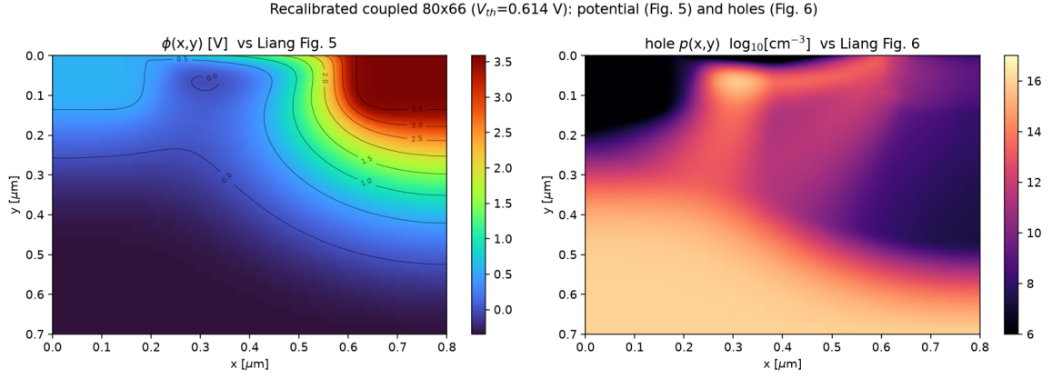
Figure 7: Potential \phi (Liang Fig. 5) and hole concentration p (Liang Fig. 6), converged Anderson 80×66: \phi rises smoothly source→drain; holes fill the p-body (II-generated holes small at the converged fixed point) and are depleted in the n^+ S/D.
