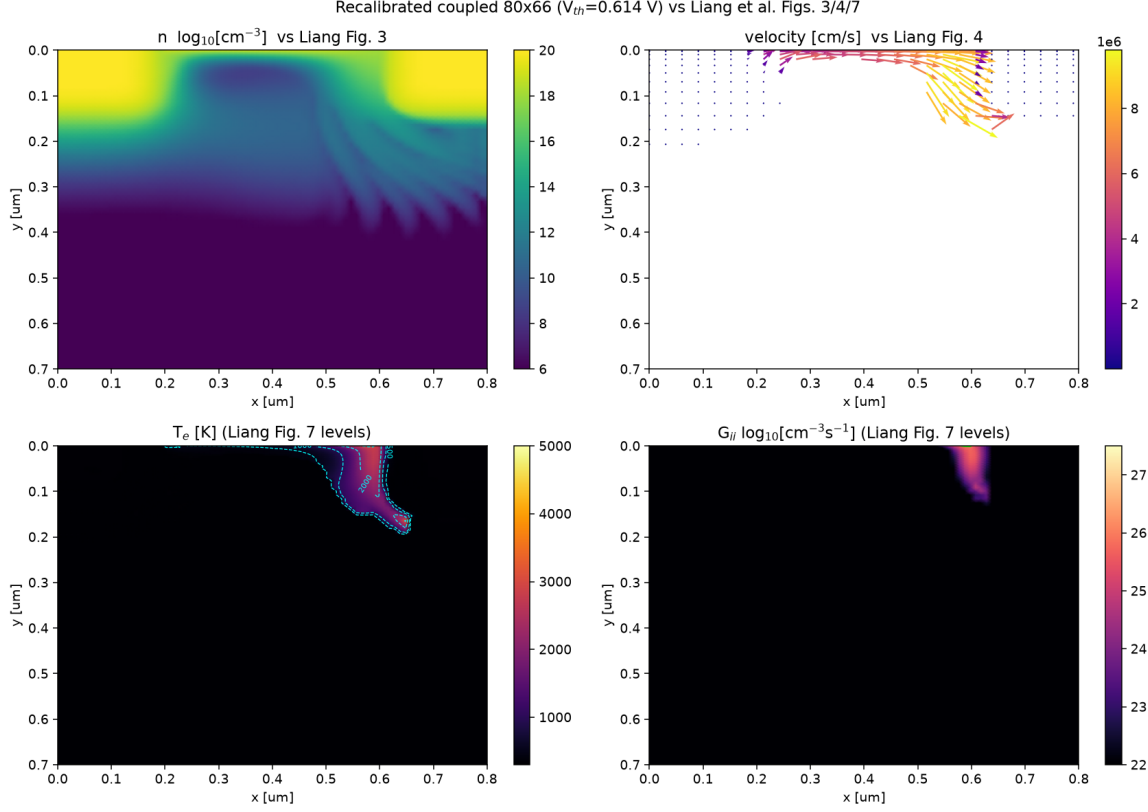
Figure 5: This work (converged Anderson 80×66) vs Liang Figs. 3 ( n ), 4 (velocity), 7 ( T_e , G_{ii} at Liang’s contour levels).
