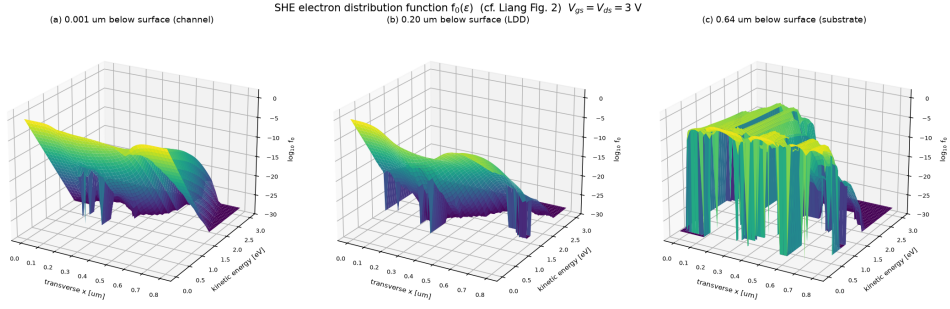
Figure 8: Energy distribution (Liang Fig. 2): a hot, non-Maxwellian tail localized at the drain surface, thermal in the bulk.
