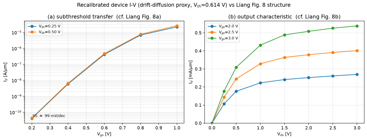
Figure 9: Terminal I-V (Liang Fig. 8), drift-diffusion proxy, per micron: (a) subthreshold transfer at V_{ds} = 0.25, 0.5 V; (b) output characteristic at V_{gs} = 2.0, 2.5, 3.0 V.
