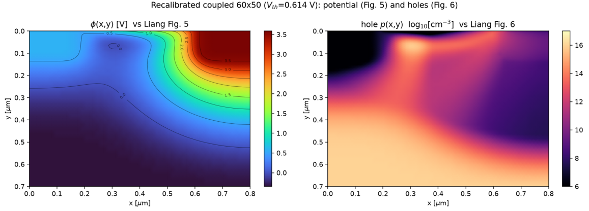
Figure 7: Potential \phi (Liang Fig. 5) and hole concentration p (Liang Fig. 6), recalibrated coupled 60 \times 50: \phi rises smoothly source \rightarrow drain; holes fill the p-body and are depleted in the n^+ S/D.
