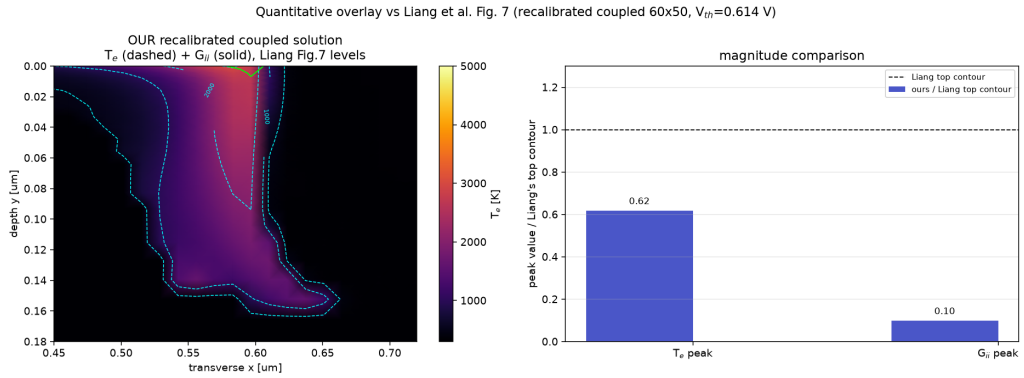
Figure 6: Quantitative Liang Fig. 7 overlay: our T_e (dashed) and G_{ii} (solid) on Liang's exact published levels; peaks reach 0.62 ( T_e ) and 0.10 ( G_{ii} , mesh-unconverged) of the top contours.
