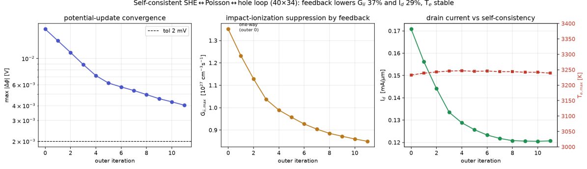
Figure 2: Self-consistent loop (40×34), first 12 damped-Picard iterations. Potential update 17.7 → 4.0 mV; feedback suppresses G_{ii} and I_d with an apparent early plateau that does not survive (Picard stalls, Fig. 3); the converged loop uses the stagnation-restart Anderson solver (§9, Fig. 4).
