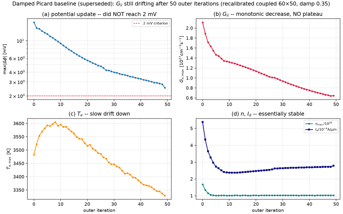
Figure 3: The damped-Picard 60 \times 50 loop stalls (50 iterations, \phi -damping 0.35 ): (a) \max|\Delta\phi| falls only to 2.5\text{ mV} ; (b) G_{ii,\max} drifts monotonically with no plateau ; (c) T_e drifts down; (d) n, I_d stable. This slow non-convergence motivated the stagnation-restart Anderson solver (Fig. 4), which reaches the fixed point Picard could not.
