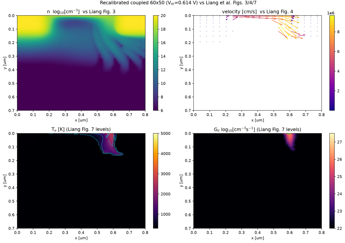
Figure 5: This work vs Liang Figs. 3 ( n ), 4 (velocity), 7 ( T_e , G_{ii} at Liang's contour levels).
