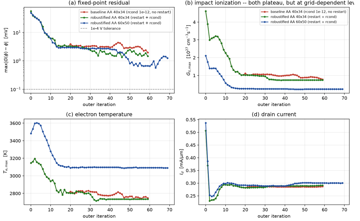
Figure 4: Stagnation-restart Anderson acceleration of the coupled loop. (a) fixed-point residual \max|G(\phi) - \phi| ; (b) G_{ii,max} ; (c) T_{e,max} ; (d) I_d . Baseline Anderson (rcond 10^{-12} , no restart; red) stalls like Picard; the restart-plus-regularized solver converges G_{ii} to a flat plateau at 40 \times 34 (green, 7.44 \times 10^{26} ) and 60 \times 50 (blue, 2.29 \times 10^{26} ). Both grids plateau, but at strongly grid-dependent levels; I_d (d) is mesh-robust.
