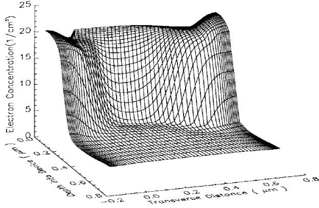
fig. 3. The calculated electron concentration for an applied bias of V_{GS} = 3 V and V_{DS} = 3 V. The electron concentration was obtained by integrating the calculated distribution function.
