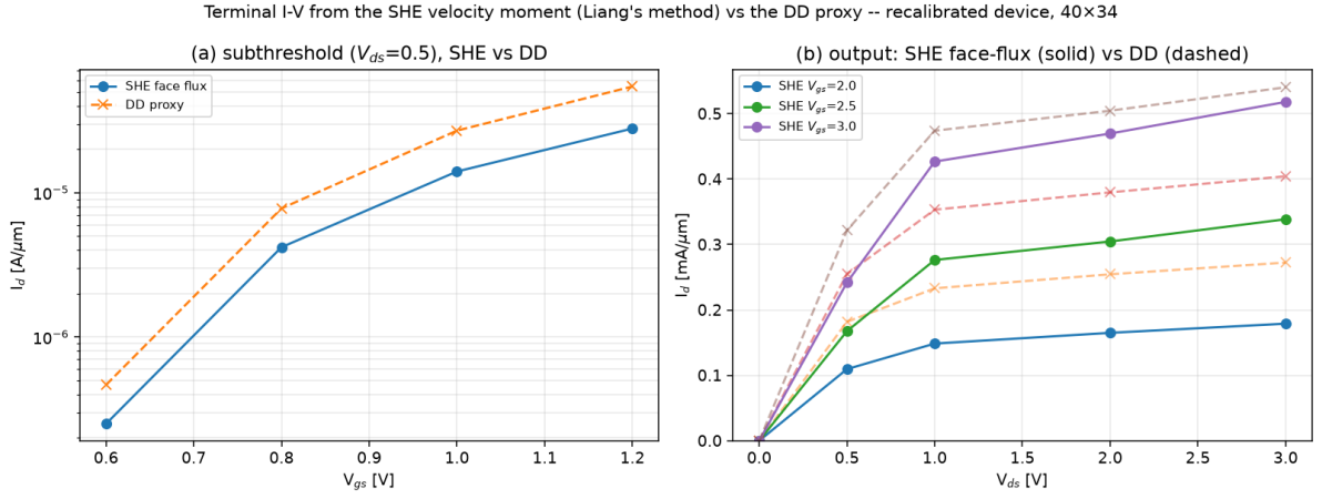
Figure 9: Terminal I-V from the SHE velocity moment (finite-volume face-flux current — Liang's method), one-way SHE on the DD potential, vs the DD proxy (dashed); recalibrated device, 40 \times 34 . (a) subthreshold ( V_{ds} = 0.5 V); (b) output families V_{gs} = 2.0, 2.5, 3.0 V. Source/drain current conservation |I_{src} + I_{drn}|/|I| is 2 \times 10^{-5} - 10^{-3} across the sweep (largest at V_{ds} = 3 V), so the reported current is the genuine SHE terminal flux. The measured ratio I_{d,SHE}/I_{d,DD} is 0.51–0.54 (subthreshold) and 0.60–0.96 (output, rising toward unity at high V_{gs}/V_{ds} ): the SHE current is systematically below the mobility-based DD proxy, consistent with the stronger nonlocal/high-field transport in the SHE solution (not attributed to a single mechanism absent a controlled diagnostic).
