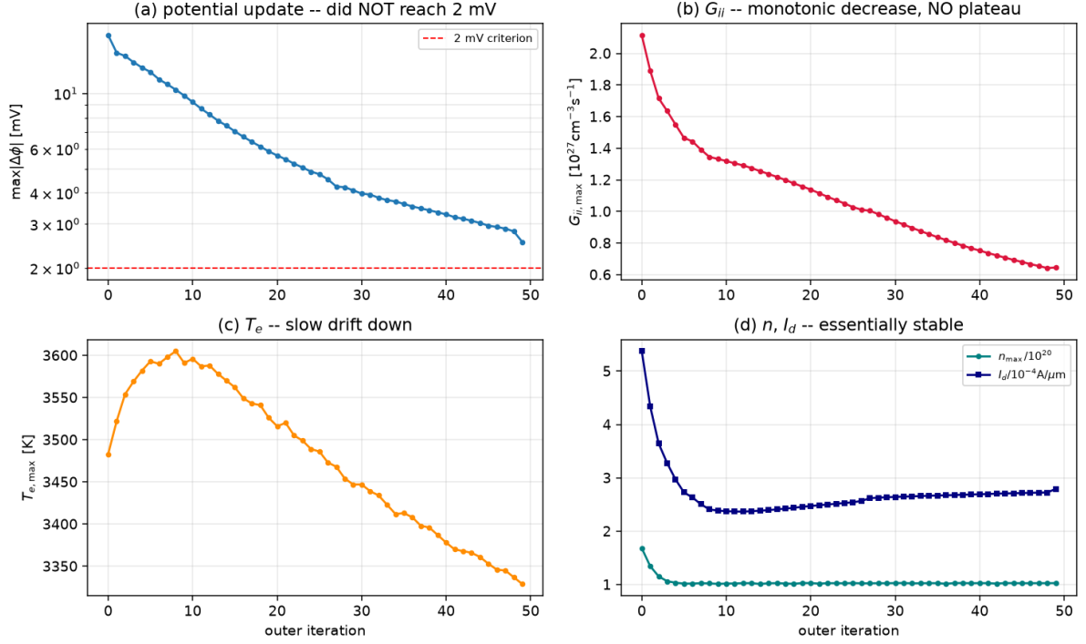
Figure 3: Recalibrated coupled 60×50 convergence study (50 outer iterations, \phi -damping 0.35). (a) \max |\Delta\phi| falls to 2.5 mV, short of the 2 mV criterion; (b) G_{ii,\max} decreases monotonically with no plateau — not converged in the outer loop; (c) T_e drifts slowly downward; (d) n and I_d are essentially stable.
