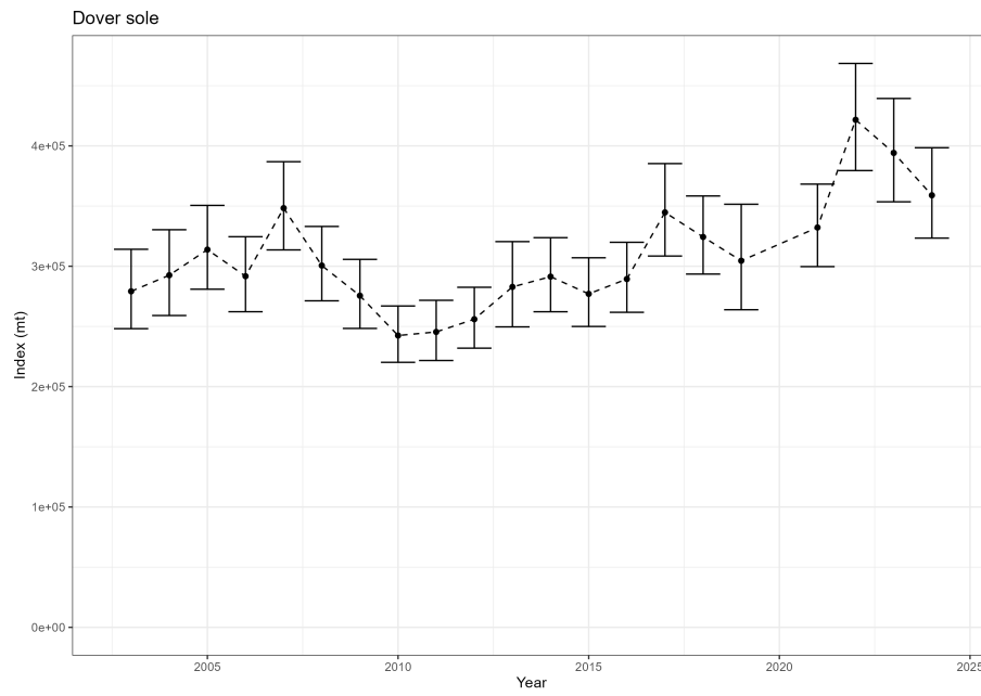
Figure 19: Estimated relative index of abundance from the NWFSC West Coast Groundfish Bottom Trawl survey.
