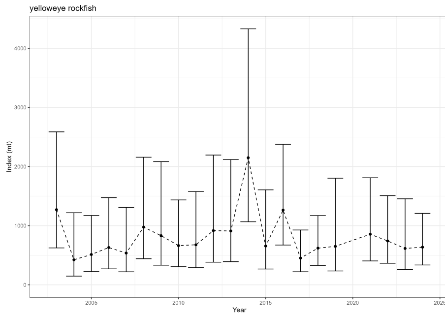
Figure 60: Estimated relative index of abundance from the NWFSC West Coast Groundfish Bottom Trawl survey.
