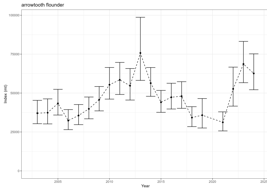
Figure 2: Estimated relative index of abundance from the NWFSC West Coast Groundfish Bottom Trawl survey.
