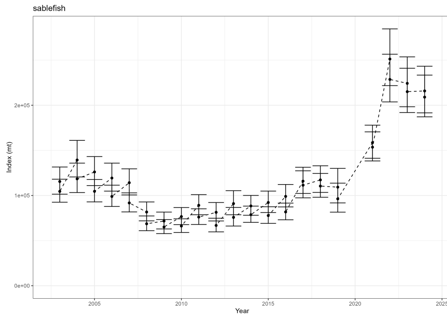
Figure 47: Estimated relative index of abundance from the NWFSC West Coast Groundfish Bottom Trawl survey.
