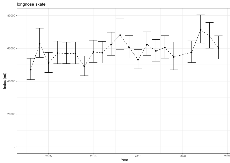
Figure 29: Estimated relative index of abundance from the NWFSC West Coast Groundfish Bottom Trawl survey.
