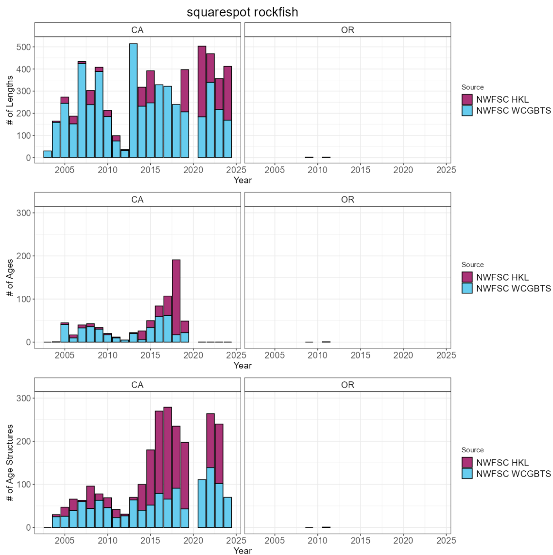
Figure 52: Total number of available lengths, read ages, and unread age structures by data source by year. Note the y-axis is unique for the number of lengths plot row compared to the number of age and age structure plot rows.
