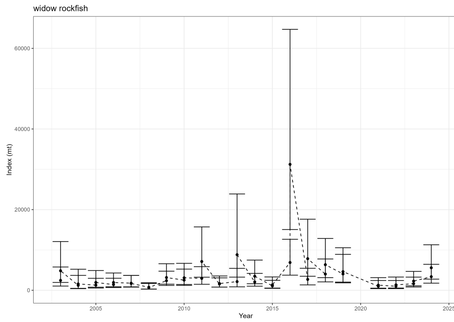
Figure 58: Estimated relative index of abundance from the NWFSC West Coast Groundfish Bottom Trawl survey.
