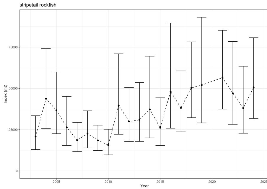
Figure 55: Estimated relative index of abundance from the NWFSC West Coast Groundfish Bottom Trawl survey.
