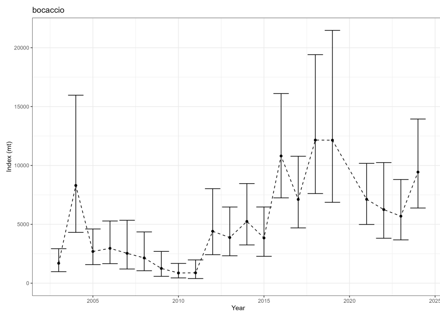
Figure 10: Estimated relative index of abundance from the NWFSC West Coast Groundfish Bottom Trawl survey.
