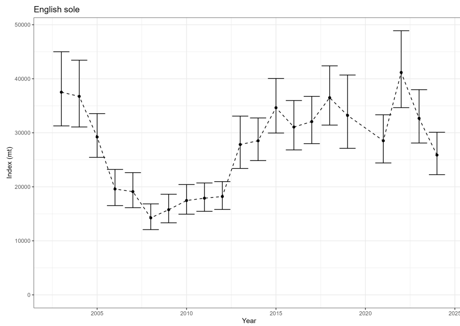
Figure 21: Estimated relative index of abundance from the NWFSC West Coast Groundfish Bottom Trawl survey.
