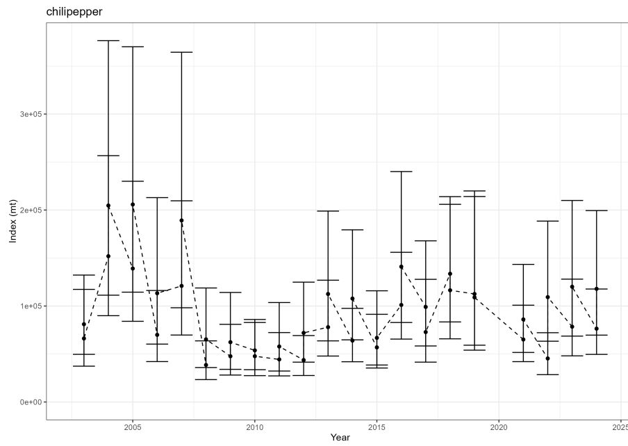
Figure 14: Estimated relative index of abundance from the NWFSC West Coast Groundfish Bottom Trawl survey.
