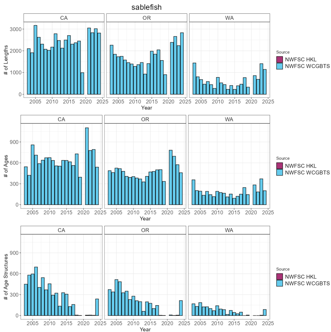
Figure 46: Total number of available lengths, read ages, and unread age structures by data source by year. Note the y-axis is unique for the number of lengths plot row compared to the number of age and age structure plot rows.
