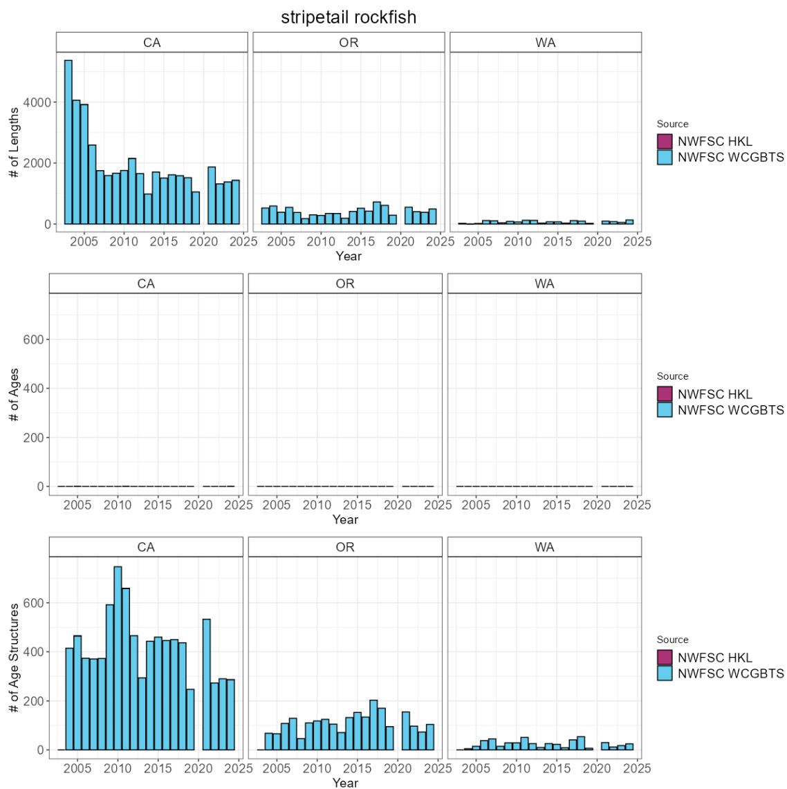
Figure 54: Total number of available lengths, read ages, and unread age structures by data source by year. Note the y-axis is unique for the number of lengths plot row compared to the number of age and age structure plot rows.
