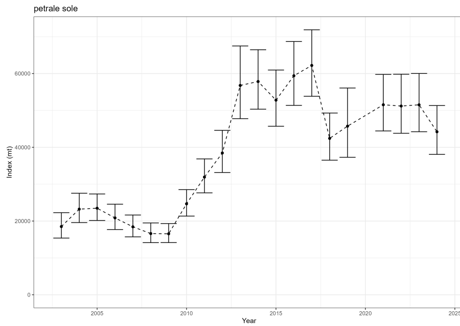
Figure 38: Estimated relative index of abundance from the NWFSC West Coast Groundfish Bottom Trawl survey.
