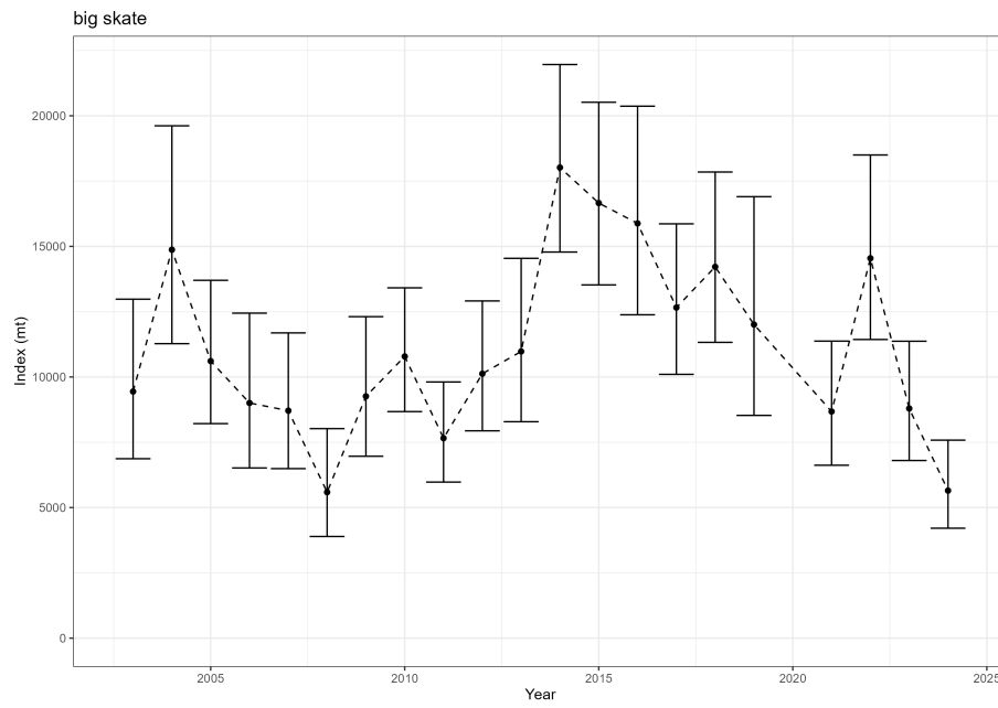
Figure 7: Estimated relative index of abundance from the NWFSC West Coast Groundfish Bottom Trawl survey.
