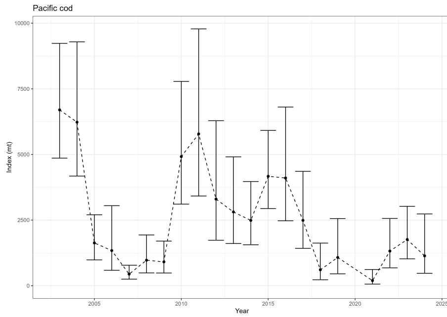
Figure 32: Estimated relative index of abundance from the NWFSC West Coast Groundfish Bottom Trawl survey.
