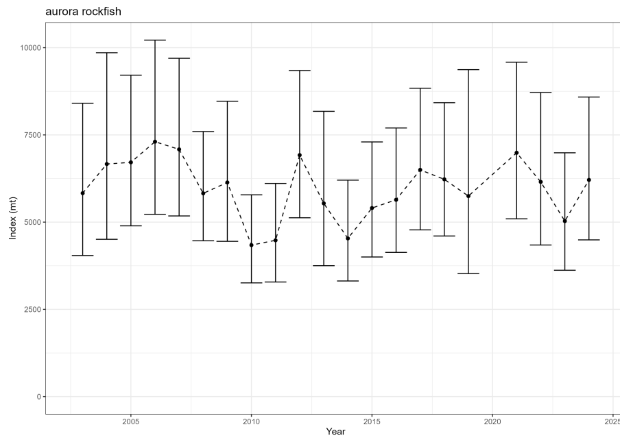
Figure 4: Estimated relative index of abundance from the NWFSC West Coast Groundfish Bottom Trawl survey.
