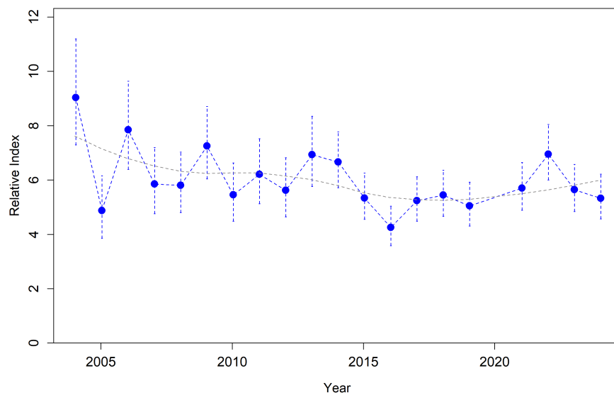
Figure 25: Estimated relative index of abundance from the NWFSC Hook and Line survey.
