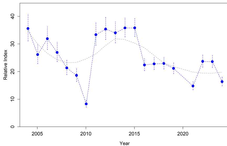
Figure 12: Estimated relative index of abundance from the NWFSC Hook and Line survey.
