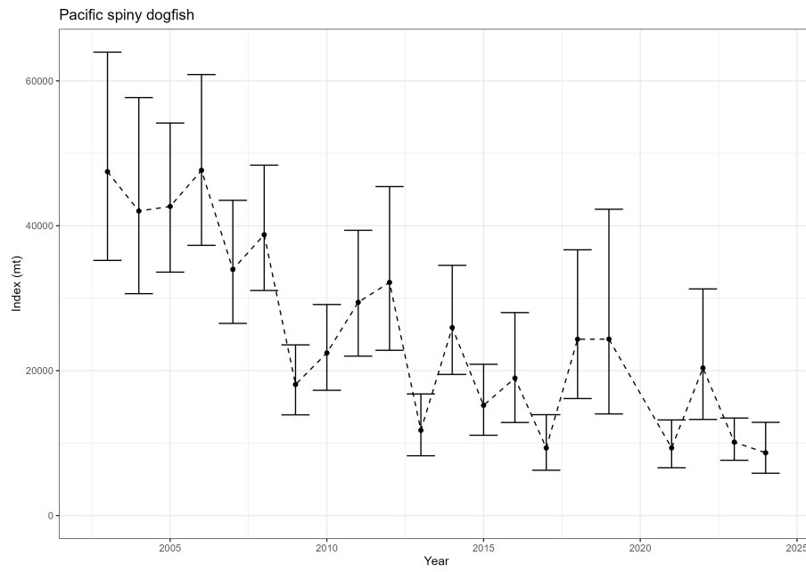
Figure 39: Estimated relative index of abundance from the NWFSC West Coast Groundfish Bottom Trawl survey.
