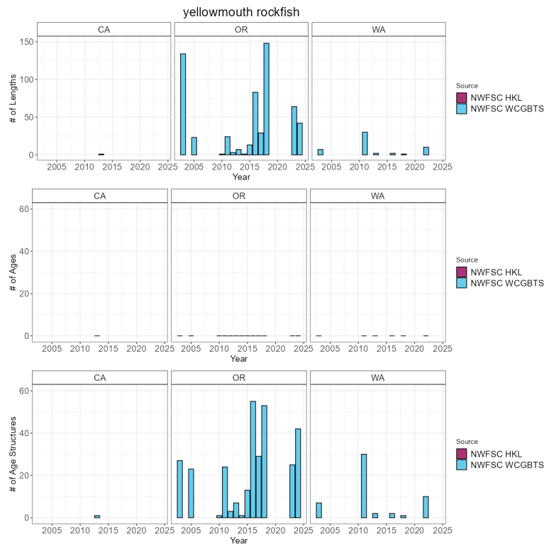
Figure 66: Total number of available lengths, read ages, and unread age structures by data source by year. Note the y-axis is unique for the number of lengths plot row compared to the number of age and age structure plot rows.
