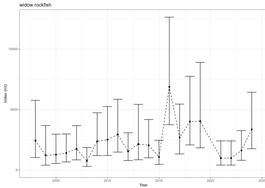
Figure 63: Estimated relative index of abundance from the NWFSC West Coast Groundfish Bottom Trawl survey.
