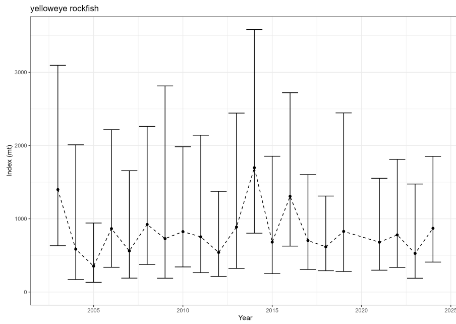
Figure 65: Estimated relative index of abundance from the NWFSC West Coast Groundfish Bottom Trawl survey.
