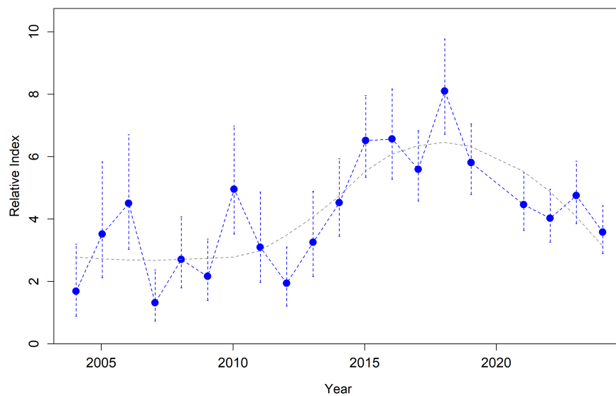
Figure 6: Estimated relative index of abundance from the NWFSC Hook and Line survey.
