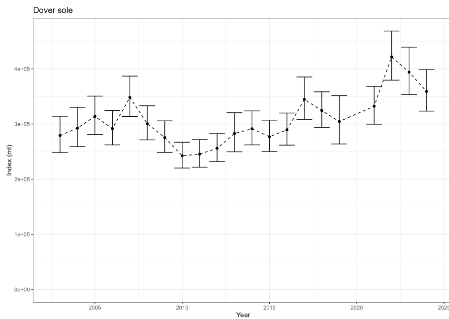
Figure 20: Estimated relative index of abundance from the NWFSC West Coast Groundfish Bottom Trawl survey.
