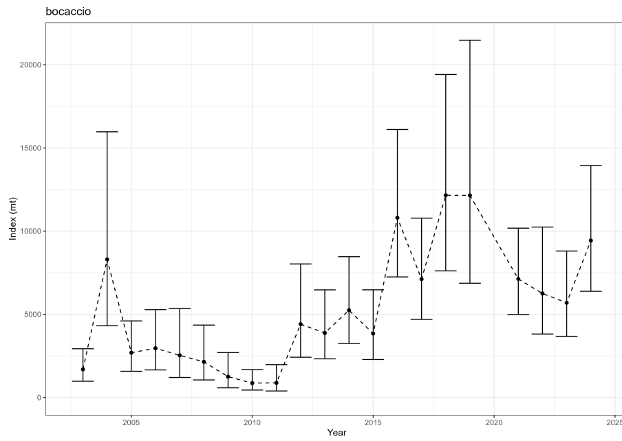
Figure 11: Estimated relative index of abundance from the NWFSC West Coast Groundfish Bottom Trawl survey.
