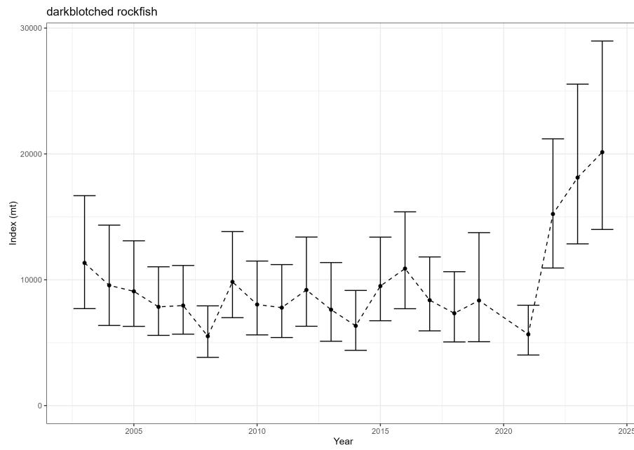
Figure 18: Estimated relative index of abundance from the NWFSC West Coast Groundfish Bottom Trawl survey.
