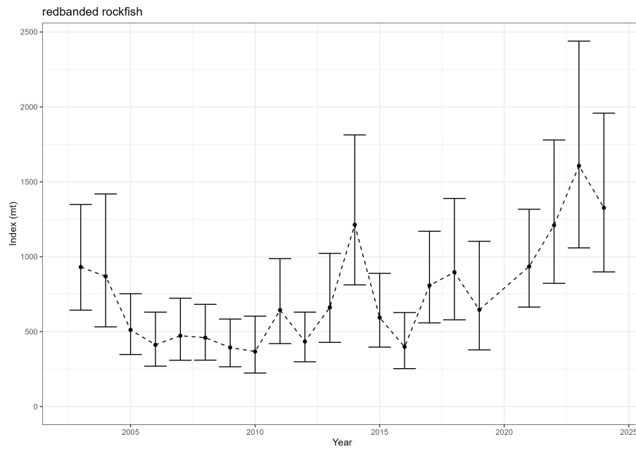
Figure 44: Estimated relative index of abundance from the NWFSC West Coast Groundfish Bottom Trawl survey.
