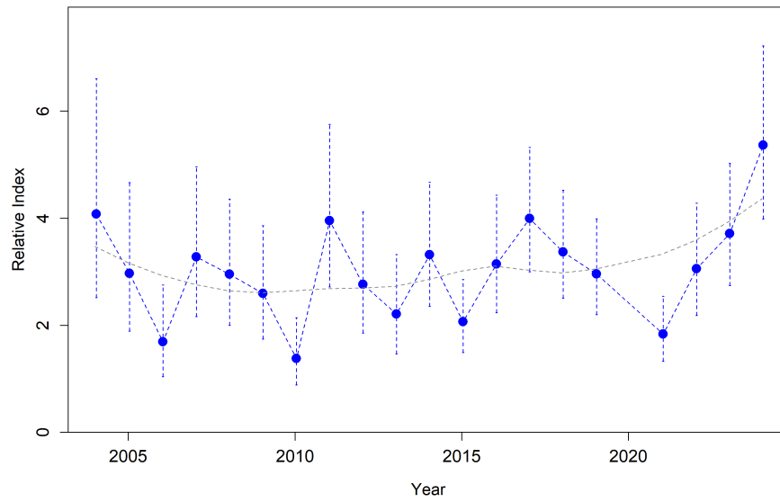
Figure 16: Estimated relative index of abundance from the NWFSC Hook and Line survey.
