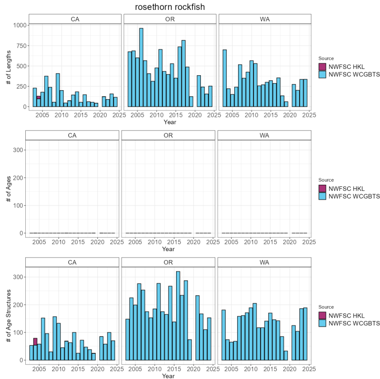
Figure 47: Total number of available lengths, read ages, and unread age structures by data source by year. Note the y-axis is unique for the number of lengths plot row compared to the number of age and age structure plot rows.
