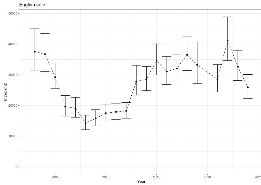
Figure 22: Estimated relative index of abundance from the NWFSC West Coast Groundfish Bottom Trawl survey.
