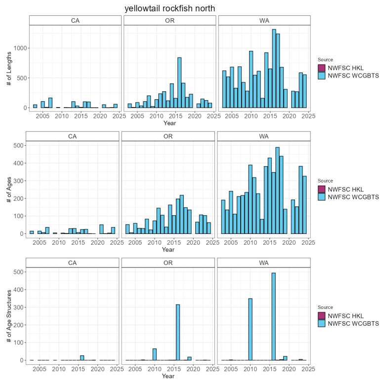
Figure 67: Total number of available lengths, read ages, and unread age structures by data source by year. Note the y-axis is unique for the number of lengths plot row compared to the number of age and age structure plot rows.
