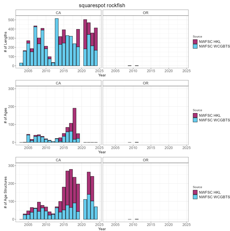
Figure 58: Total number of available lengths, read ages, and unread age structures by data source by year. Note the y-axis is unique for the number of lengths plot row compared to the number of age and age structure plot rows.
