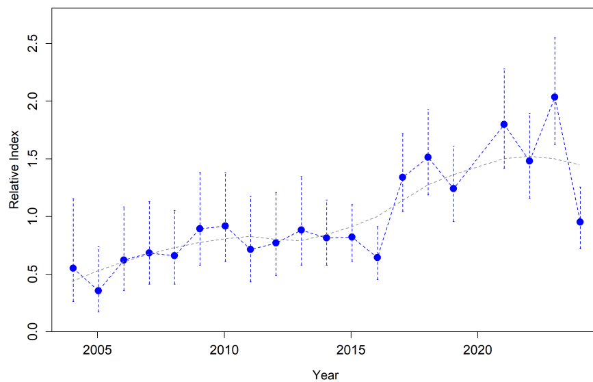
Figure 29: Estimated relative index of abundance from the NWFSC Hook and Line survey.
