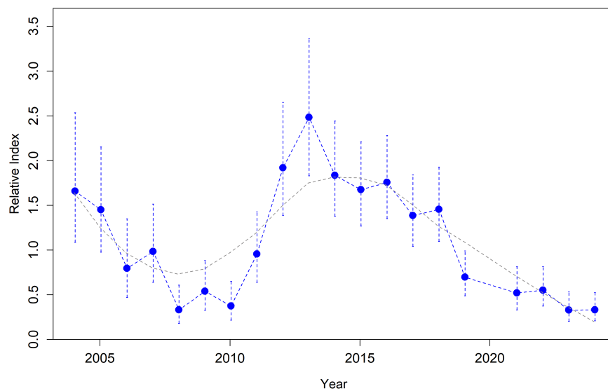
Figure 33: Estimated relative index of abundance from the NWFSC Hook and Line survey.
