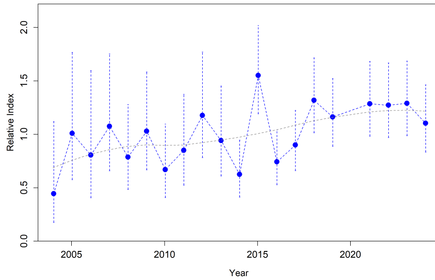
Figure 18: Estimated relative index of abundance from the NWFSC Hook and Line survey.
