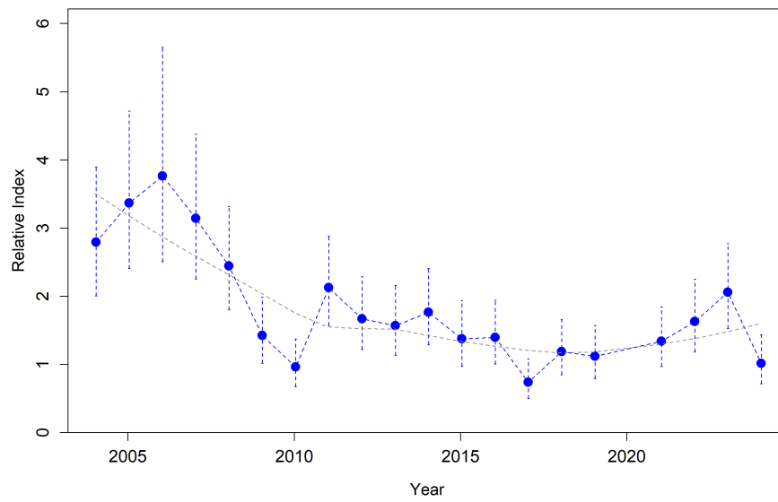
Figure 73: Estimated relative index of abundance from the NWFSC Hook and Line survey.
