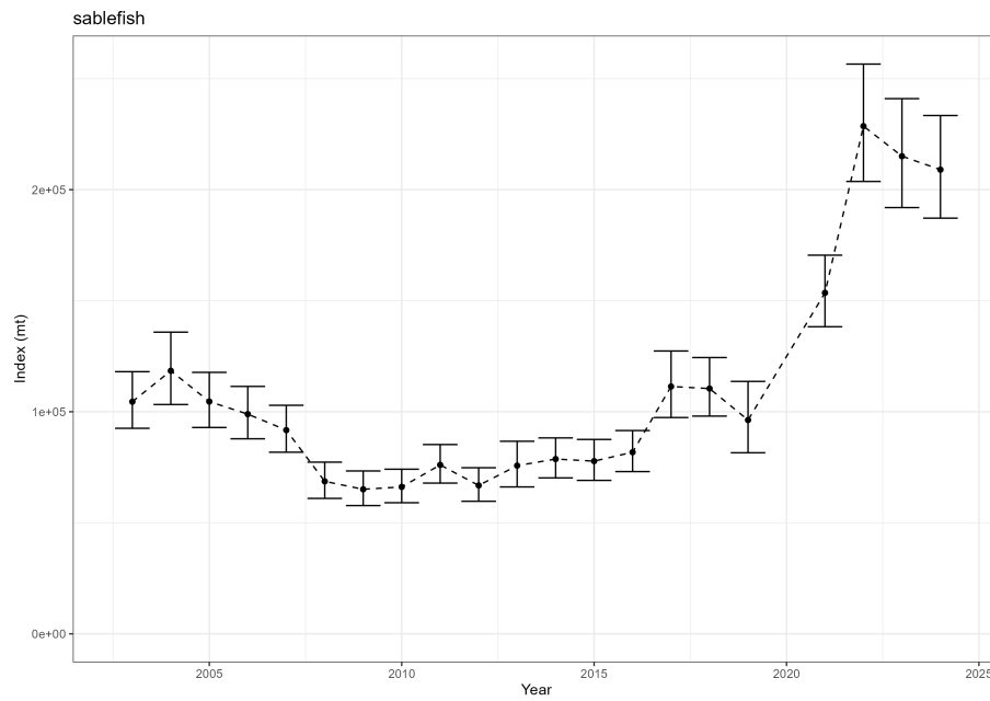
Figure 53: Estimated relative index of abundance from the NWFSC West Coast Groundfish Bottom Trawl survey.
