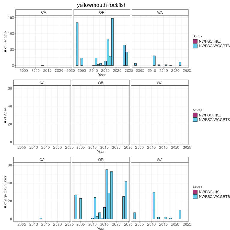
Figure 70: Total number of available lengths, read ages, and unread age structures by data source by year. Note the y-axis is unique for the number of lengths plot row compared to the number of age and age structure plot rows.
