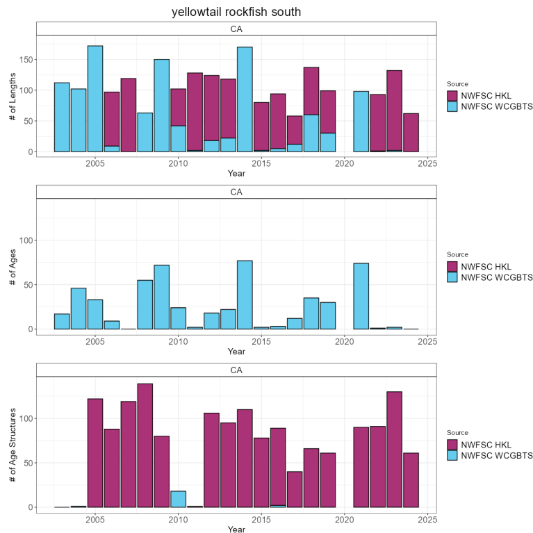
Figure 72: Total number of available lengths, read ages, and unread age structures by data source by year. Note the y-axis is unique for the number of lengths plot row compared to the number of age and age structure plot rows.
