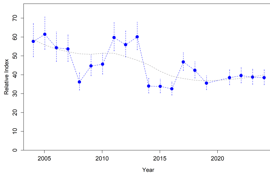
Figure 65: Estimated relative index of abundance from the NWFSC Hook and Line survey.
