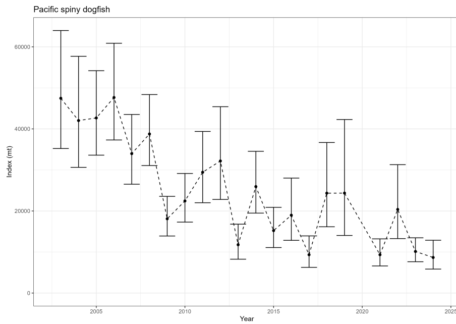
Figure 42: Estimated relative index of abundance from the NWFSC West Coast Groundfish Bottom Trawl survey.
