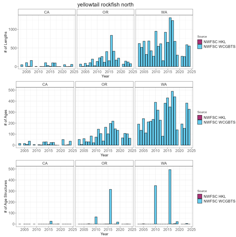
Figure 71: Total number of available lengths, read ages, and unread age structures by data source by year. Note the y-axis is unique for the number of lengths plot row compared to the number of age and age structure plot rows.
