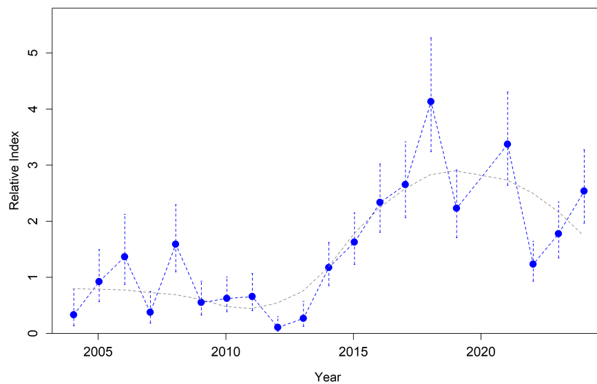
Figure 59: Estimated relative index of abundance from the NWFSC Hook and Line survey.
