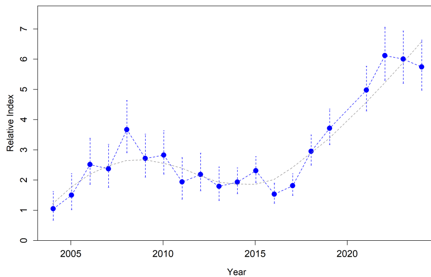
Figure 61: Estimated relative index of abundance from the NWFSC Hook and Line survey.
