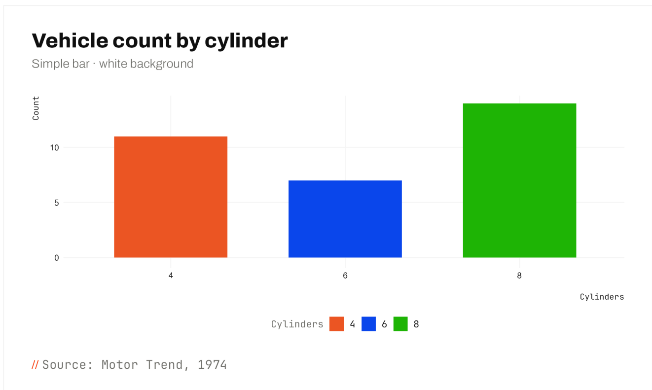
FIGURE 6 · VEHICLE COUNT BY CYLINDER CLASS.
