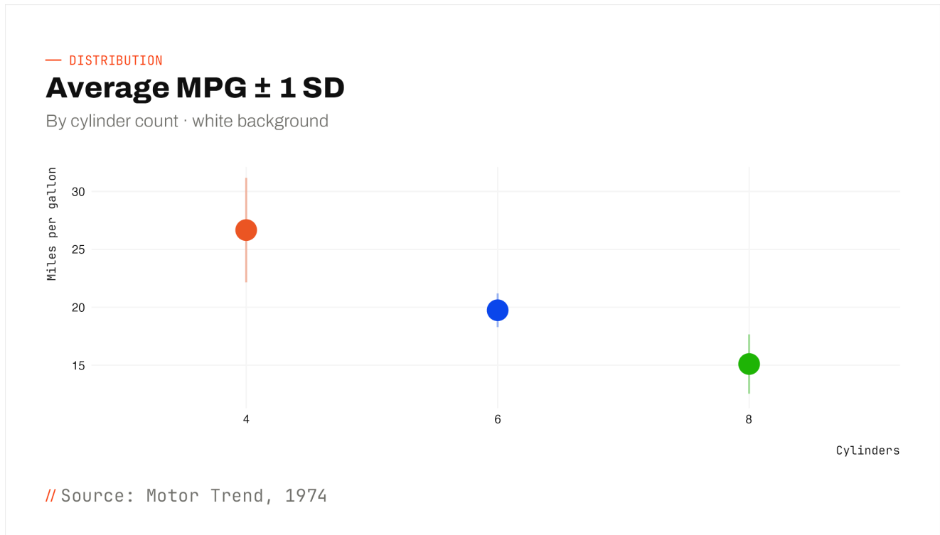
FIGURE 10 · LOLLIPOP — AVERAGE MPG WITH \pm 1 SD ERROR, BY CYLINDER.
