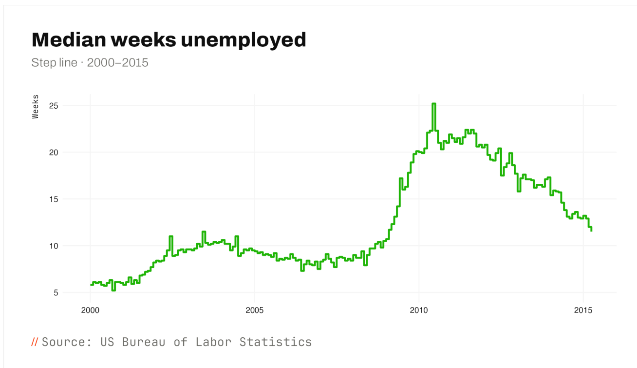
FIGURE 14 · STEP CHART — MEDIAN UNEMPLOYMENT DURATION.
