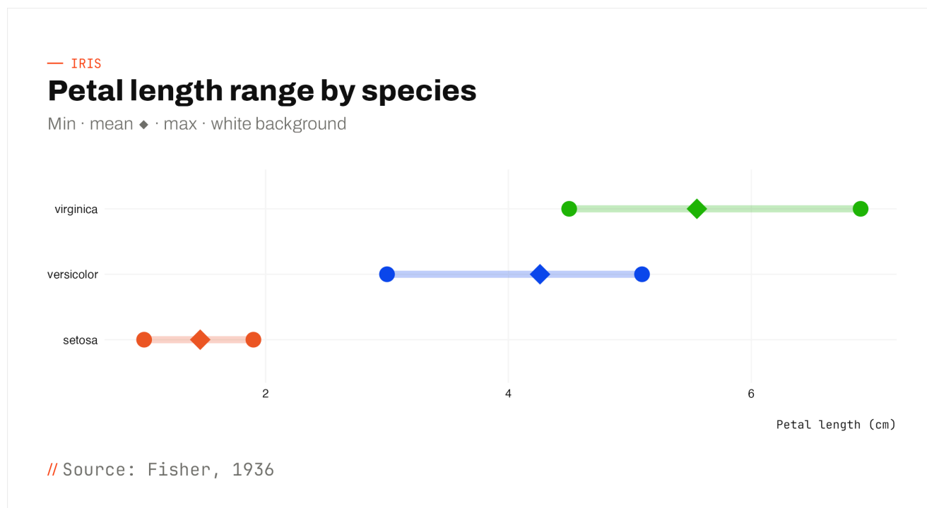
FIGURE 23 · RANGE PLOT — PETAL LENGTH MIN/MAX/MEAN BY SPECIES.
