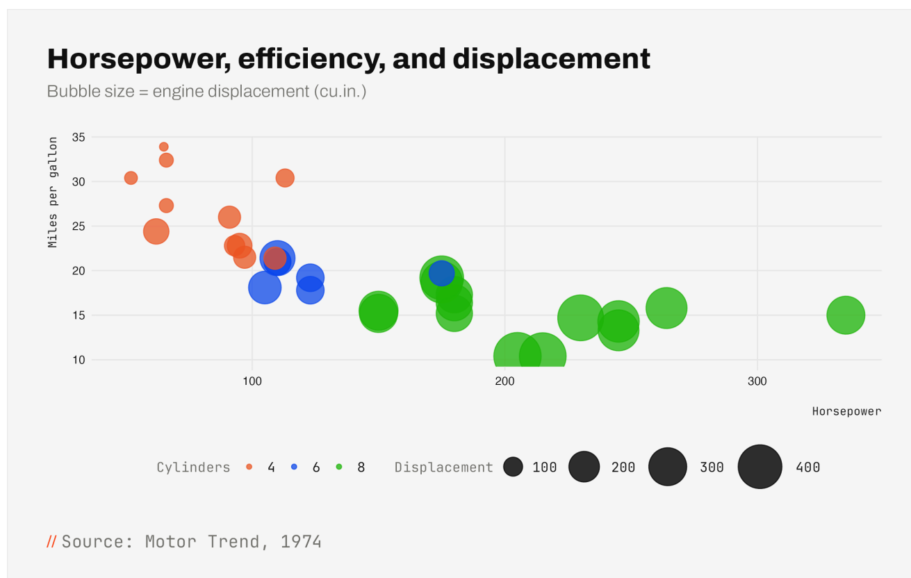
FIGURE 4 • BUBBLE CHART — ENGINE DISPLACEMENT DRIVES POINT SIZE.
