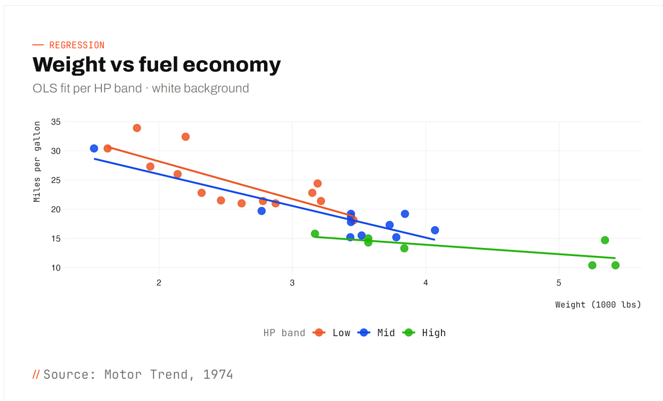
FIGURE 3 · SCATTER WITH PER-GROUP OLS LINES. HP BAND DRIVES COLOUR.
