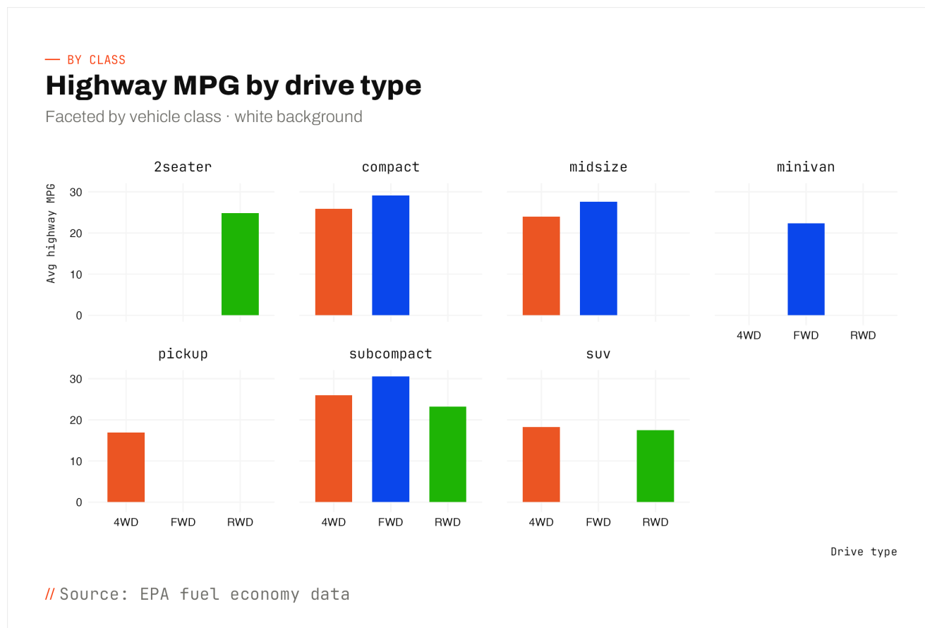
FIGURE 21 · FACETED BAR — HIGHWAY MPG BY DRIVE TYPE, FACETED BY VEHICLE CLASS.
