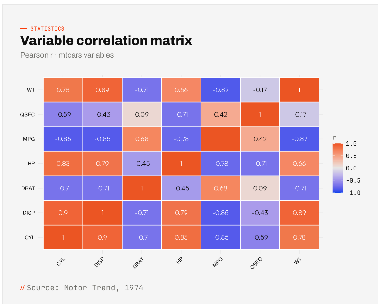
FIGURE 18 • PEARSON CORRELATION MATRIX FOR SELECTED MTCARS VARIABLES.
