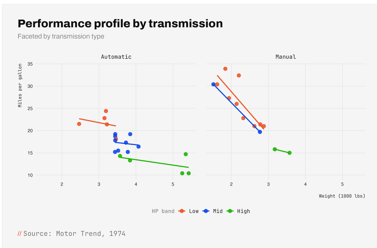
FIGURE 20 • FACETED SCATTER WITH REGRESSION LINES – TRANSMISSION TYPE PANELS.
