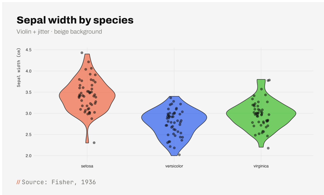
FIGURE 17 · VIOLIN PLOT OF SEPAL WIDTH BY SPECIES WITH RAW DATA OVERLAY.
