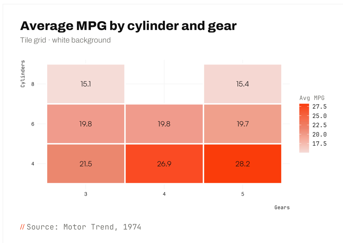
FIGURE 19 • AVERAGE MPG TILE GRID — CYLINDER × GEAR COMBINATIONS.
