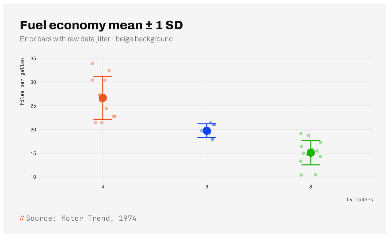
FIGURE 22 • MEAN MPG \pm 1 SD WITH INDIVIDUAL OBSERVATIONS OVERLAID.
