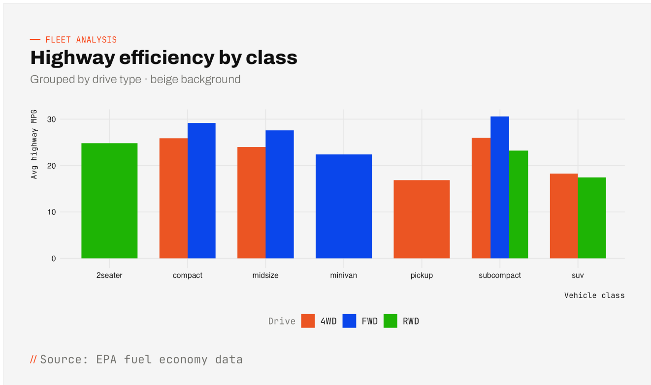
FIGURE 7 • AVERAGE HIGHWAY MPG BY VEHICLE CLASS AND DRIVE TYPE.
