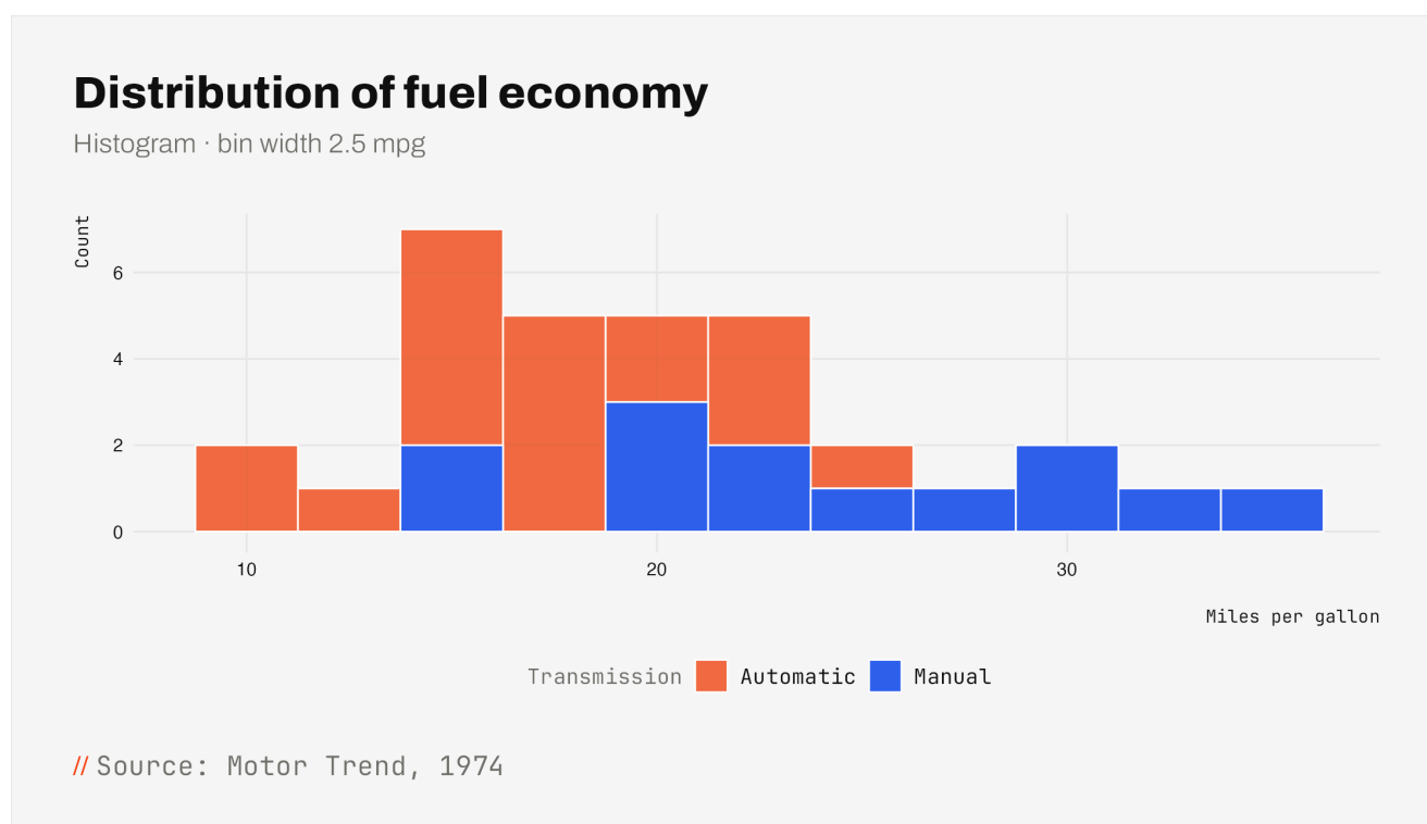
FIGURE 15 · HISTOGRAM OF FUEL ECONOMY (MPG) ACROSS ALL VEHICLES.
