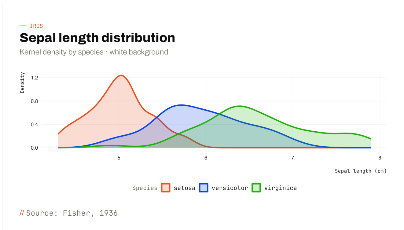
FIGURE 16 · KERNEL DENSITY OF SEPAL LENGTH BY IRIS SPECIES.
