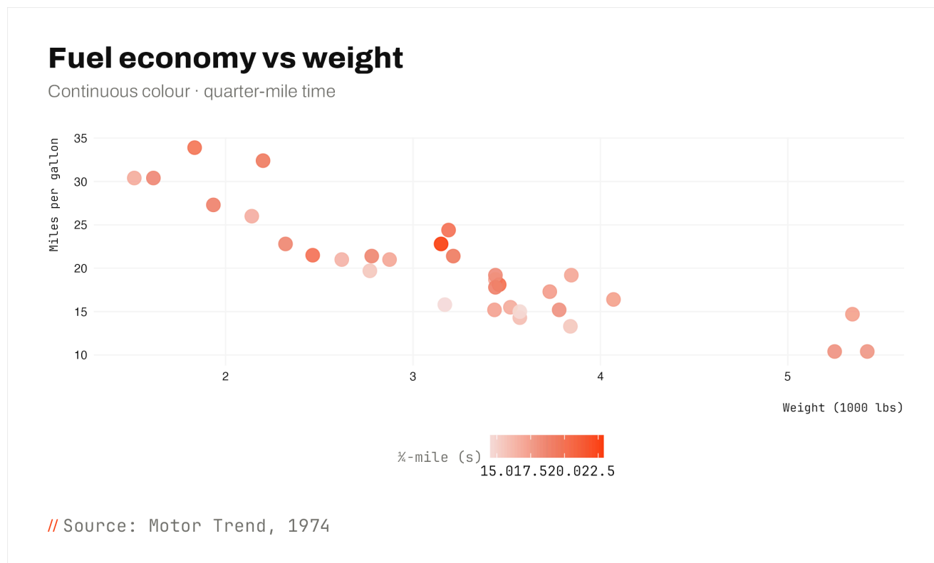
FIGURE 5 · SCATTER WITH CONTINUOUS COLOUR GRADIENT — QUARTER-MILE TIME.
